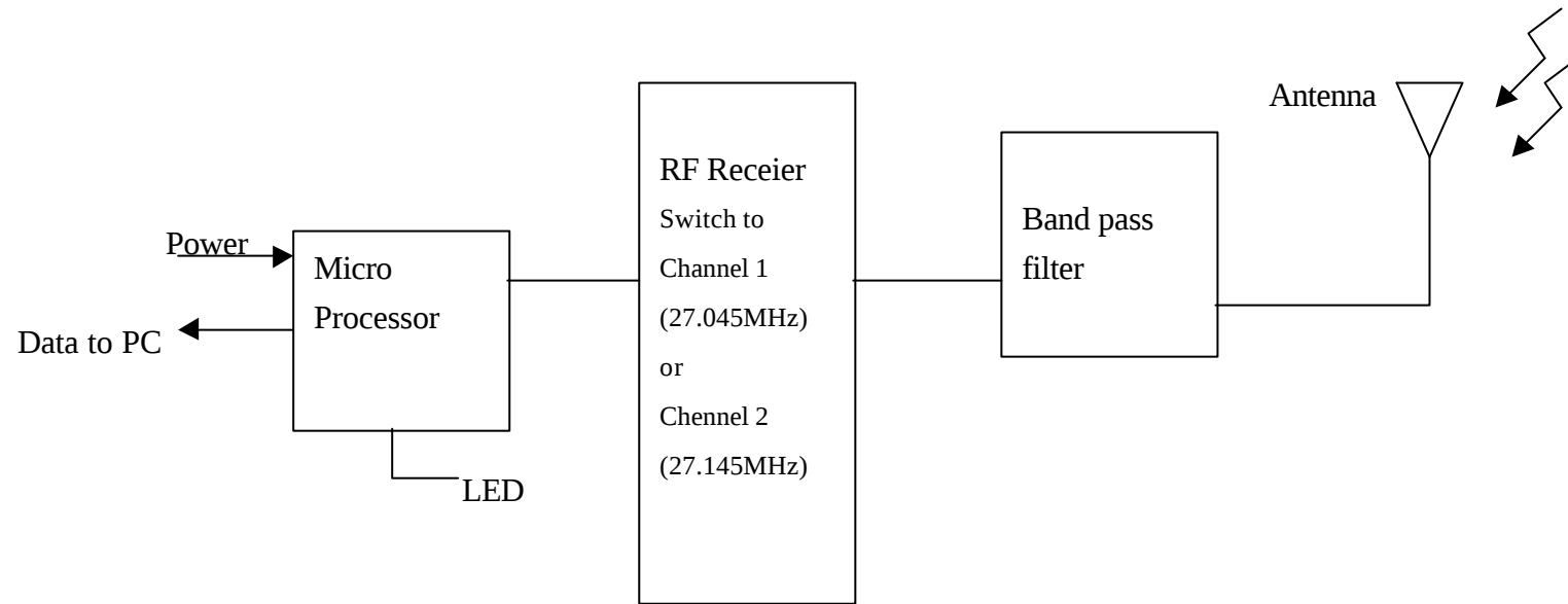
Model: RFRX5 and RFRX5PU (Receiver)
