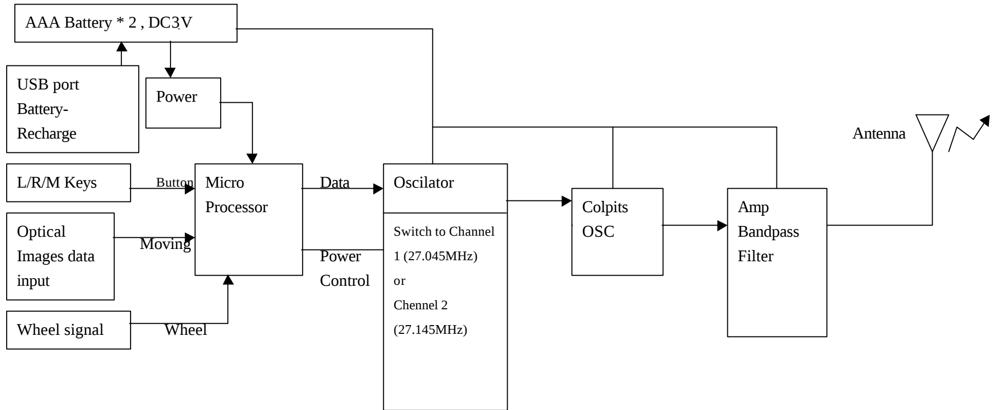
RFSOP-29 Wireless Mouse (Transmitter)
