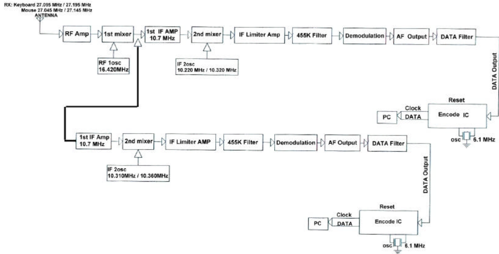
Receicer Block Diagram
