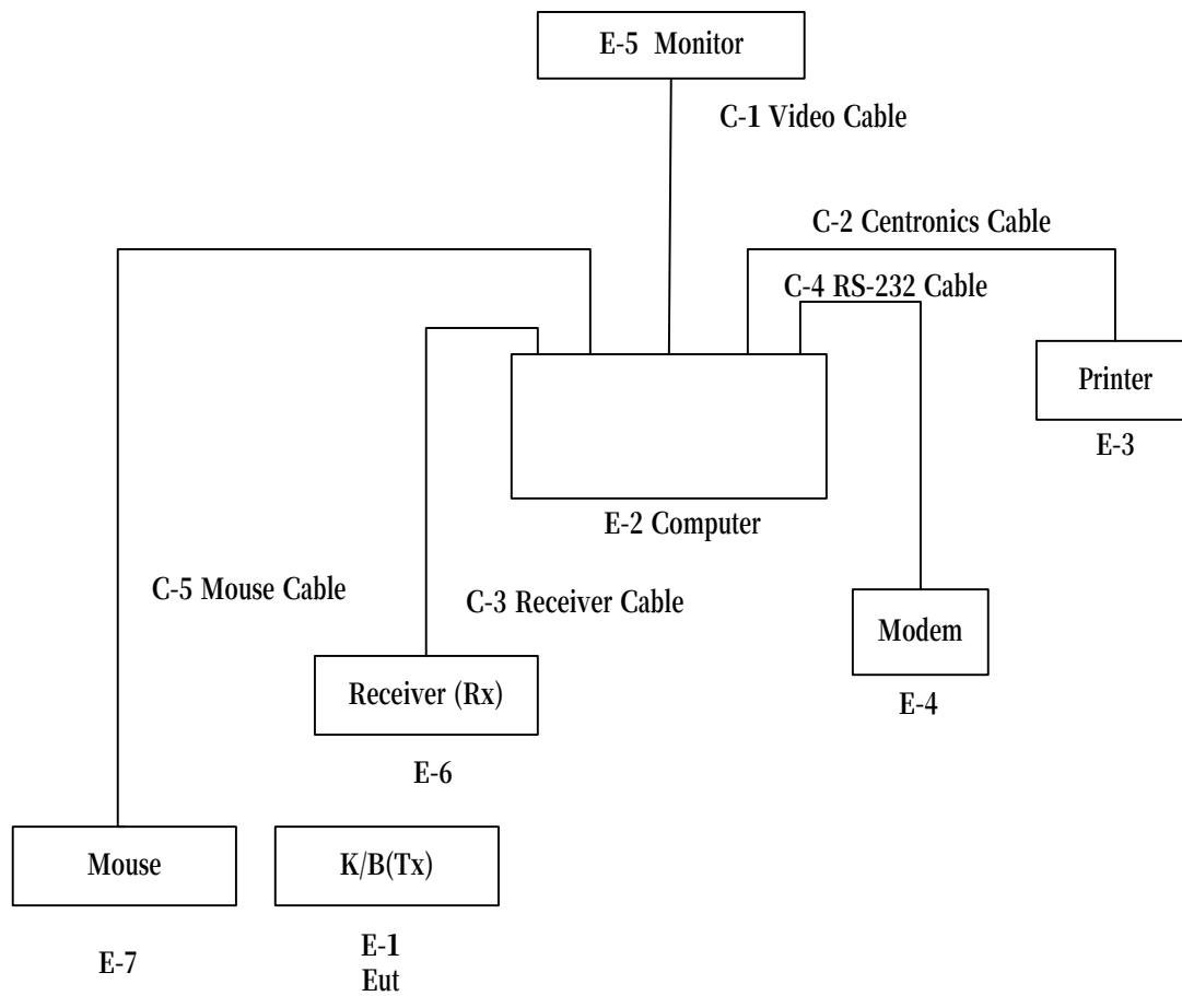
Diagram - 1 Block diagram showing the configuration of system tested
