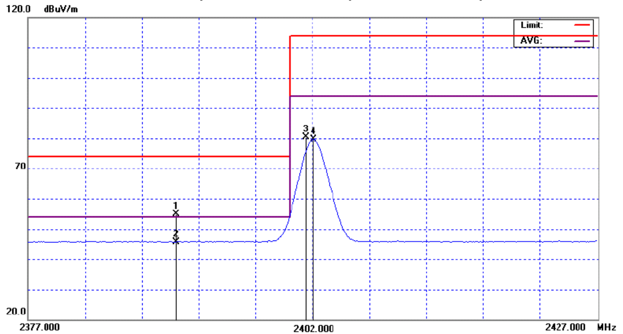
TX CH01 (Restricted Bands Requirements, Vertical)
