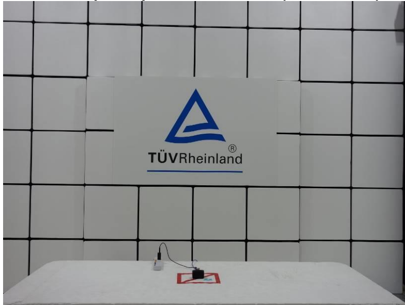
Photograph 2: Test Setup for Spurious Emissions (Front View 2)
