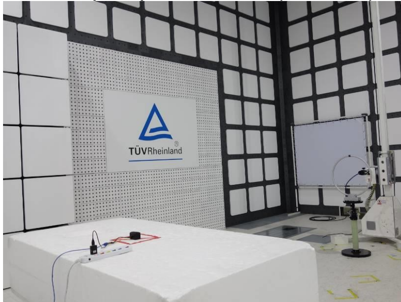
Photograph 4: Test Setup for Spurious Emissions (Back View 2)
