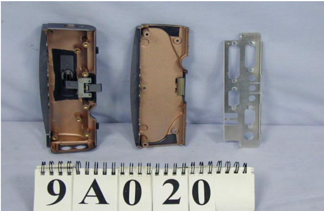
EUT Case Inside View
