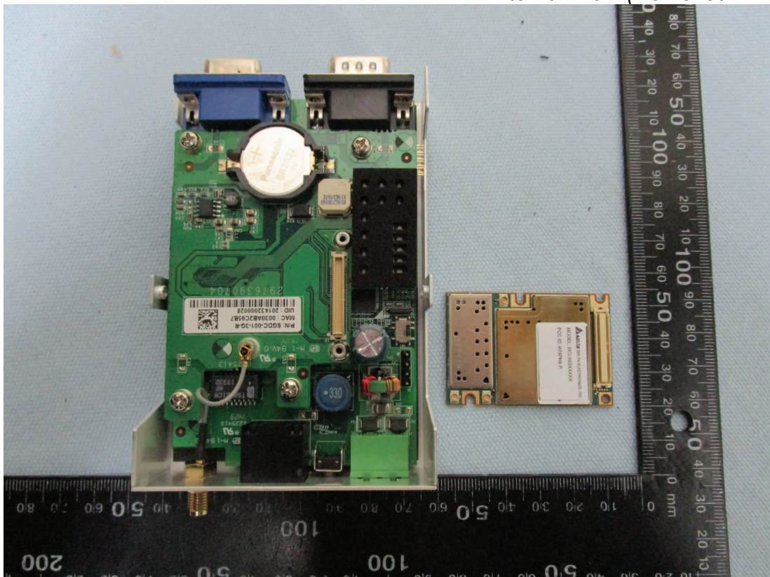
Figure 7 Internal View (Removed RF Module)
