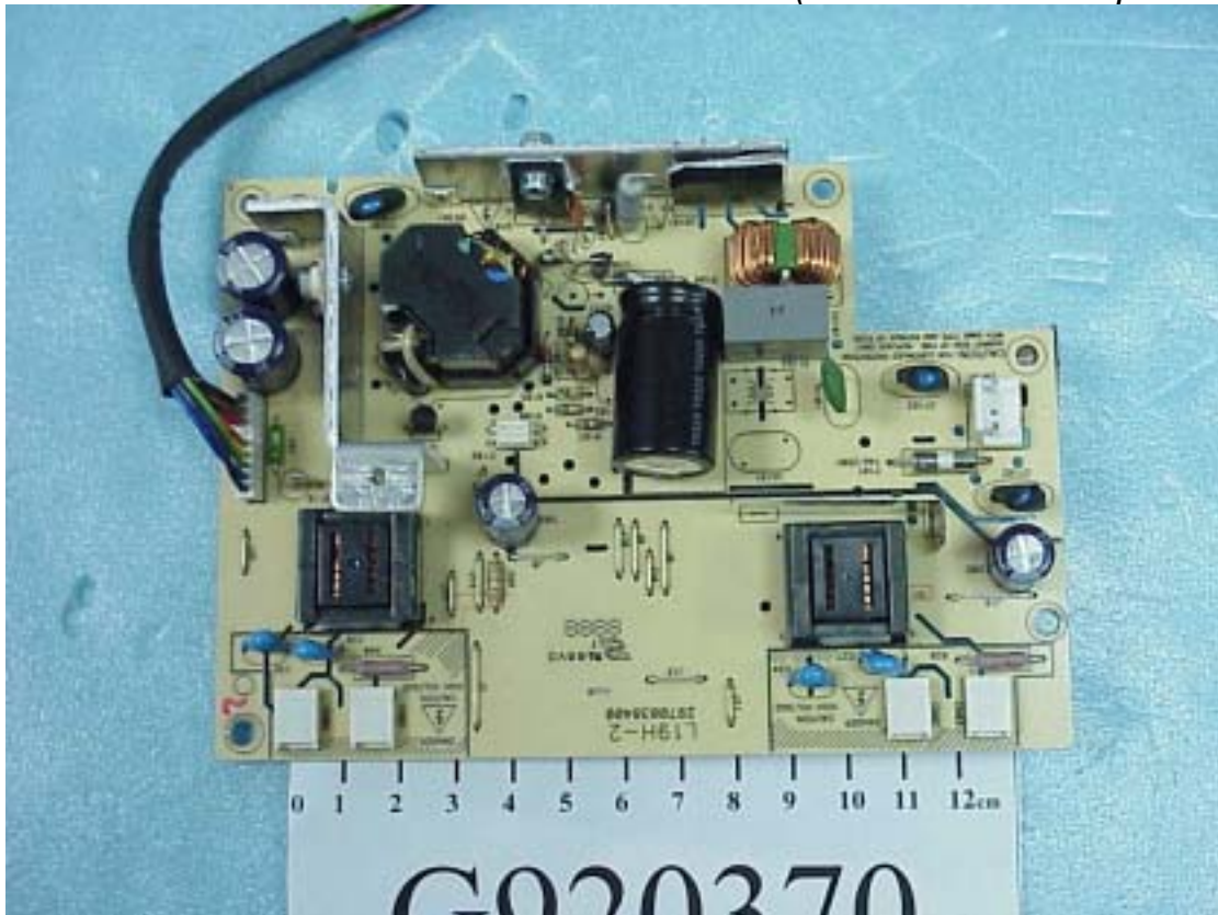
Figure 9 Internal View (Power Board/Component Side)
