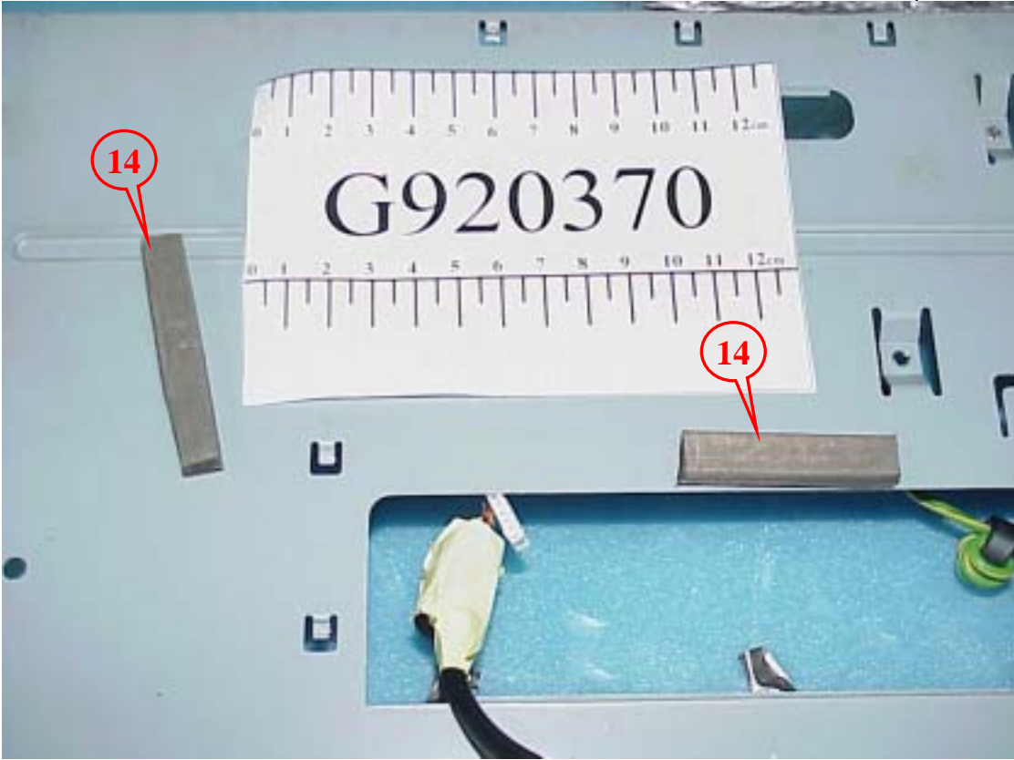
Figure 26 Internal View (EMI Solution)
