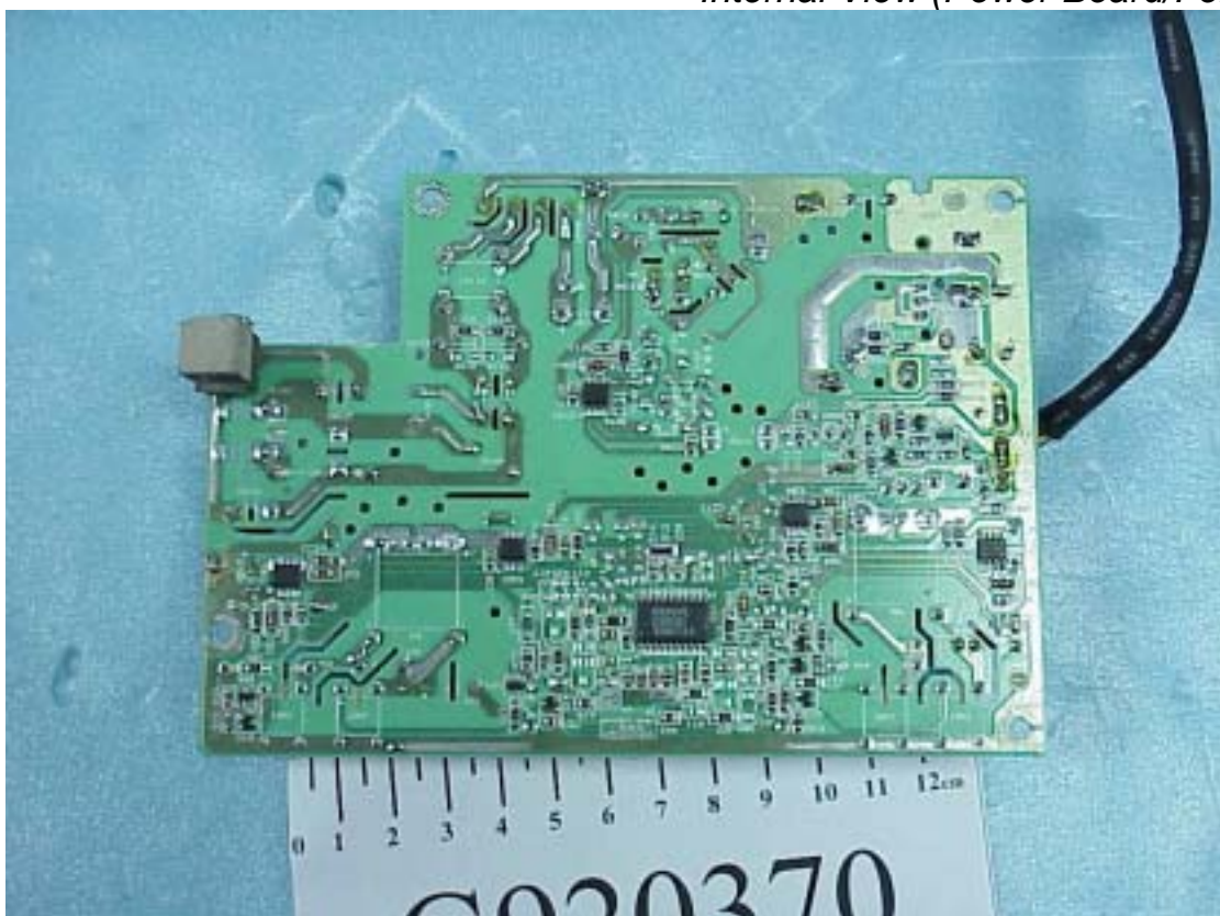
Figure 10 Internal View (Power Board/Foil Side)
