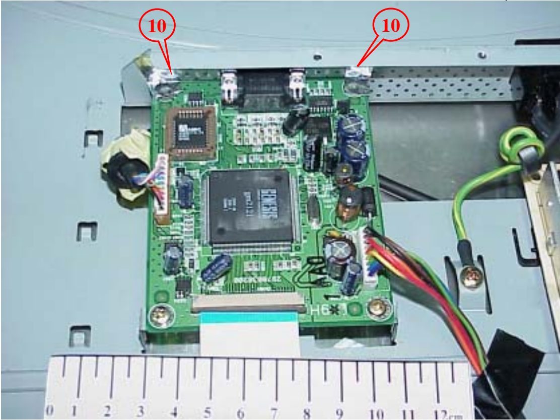
Figure 22 Internal View (EMI Solution)
