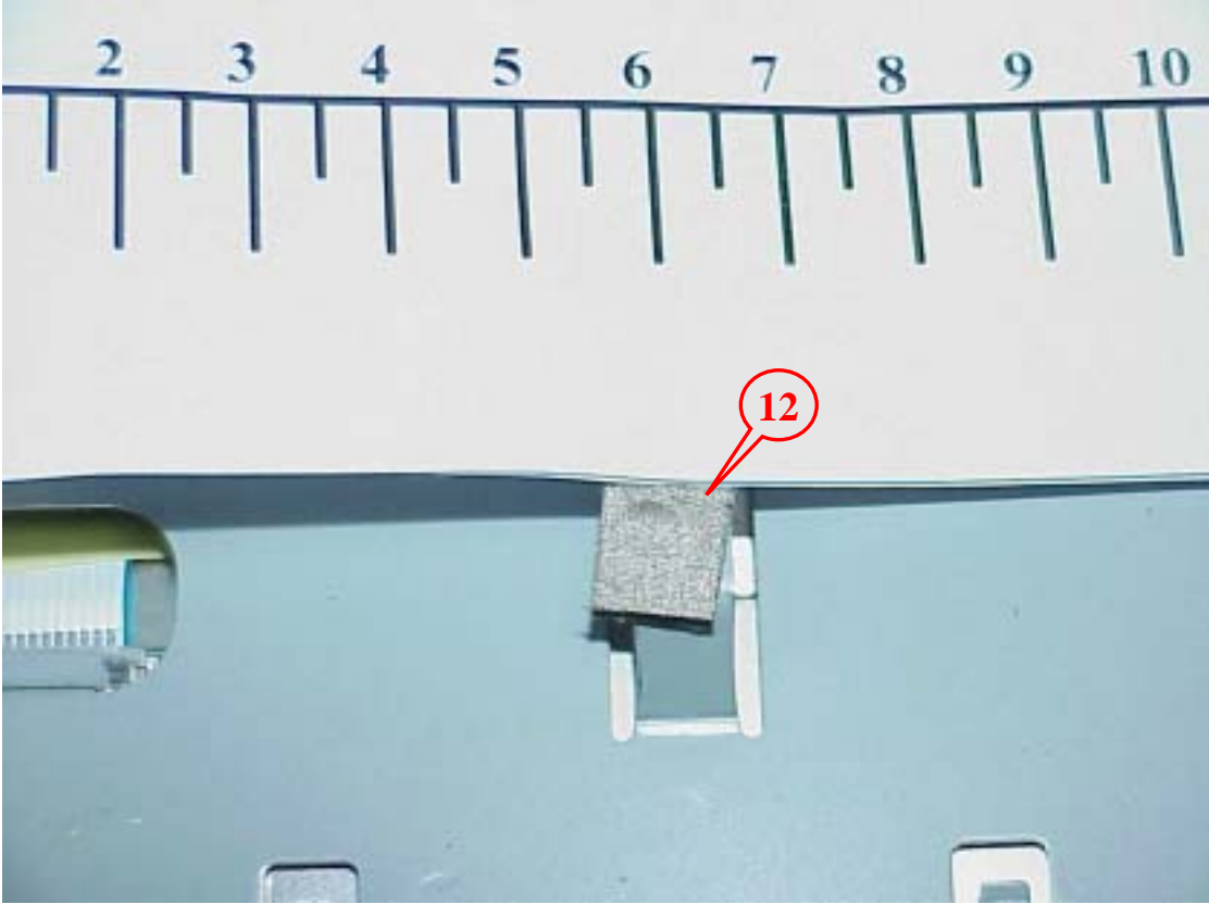
Figure 24 Internal View (EMI Solution)
