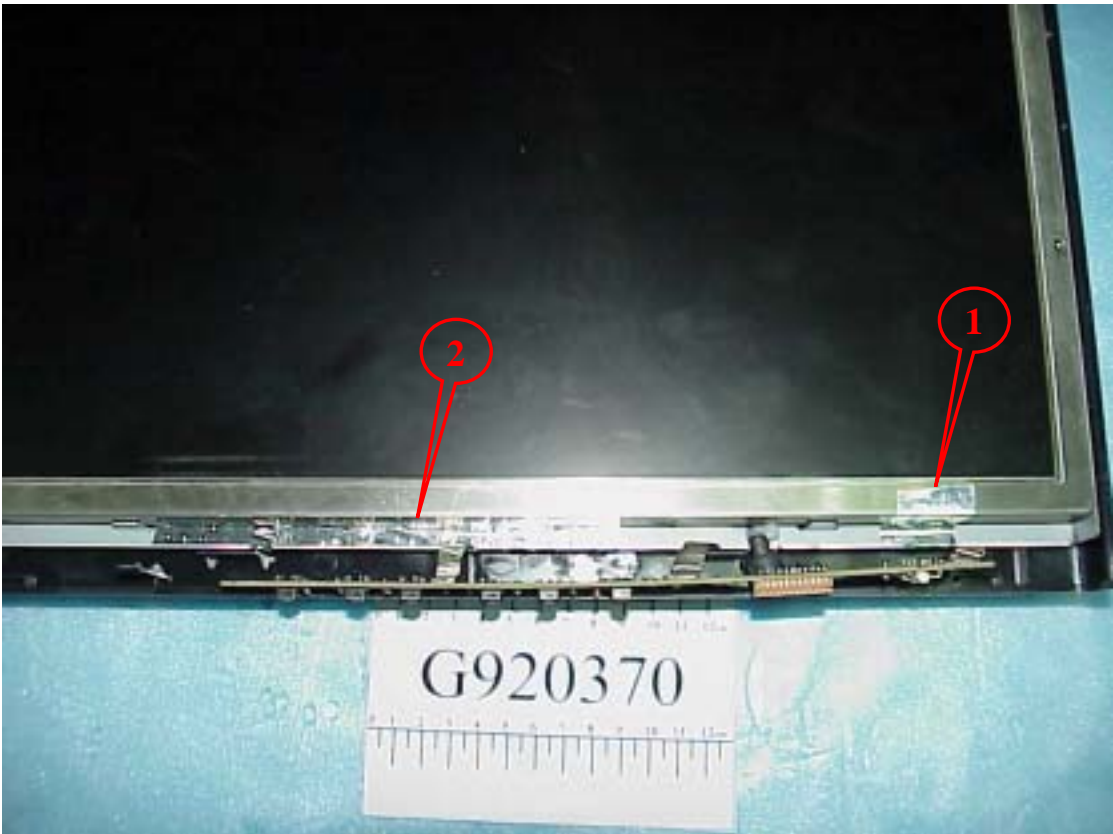
Figure 20 Data Cable
