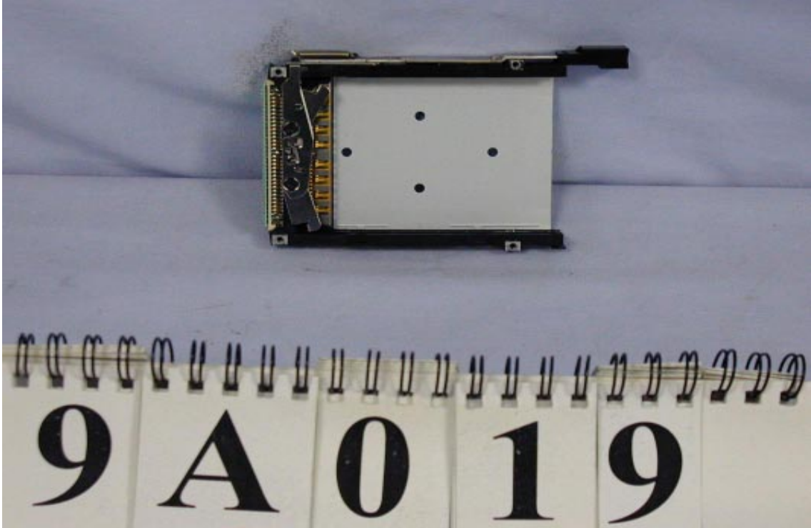
PCMCIA Slot Component Side View
