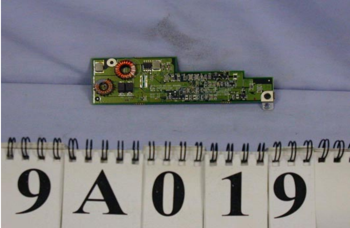
DC To DC Board Component Side View
