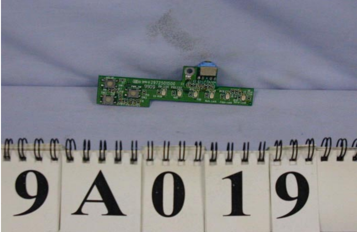
Control Board Component Side View
