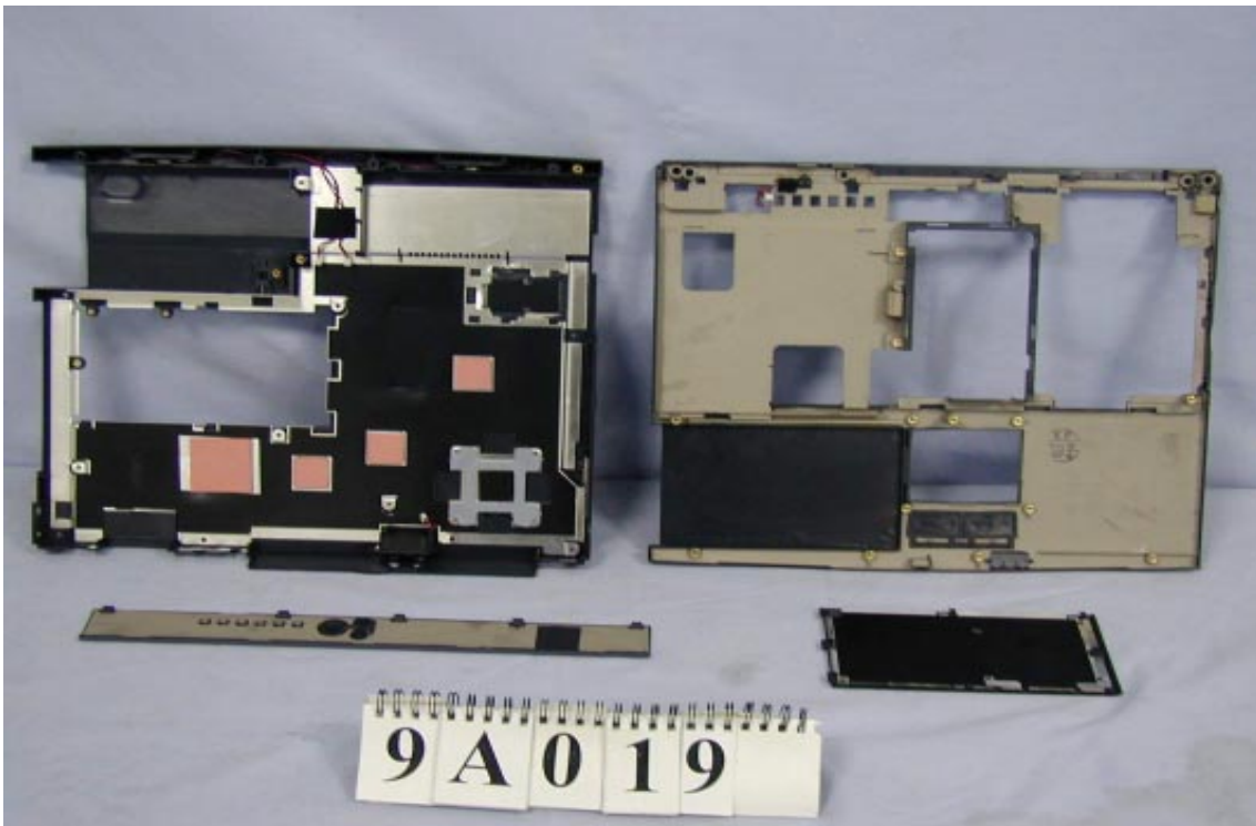
EUT Case Inside View
