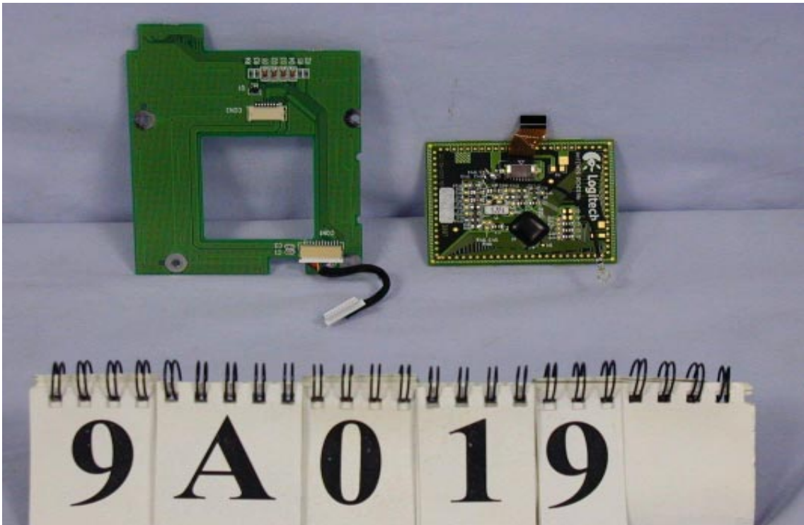
Mouse Board Solder Side View
