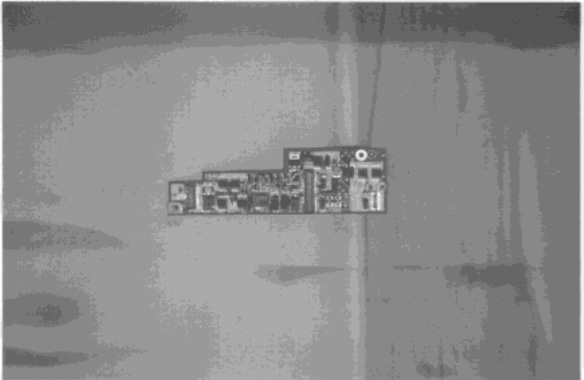
DC to DC Converter Solder Side View
