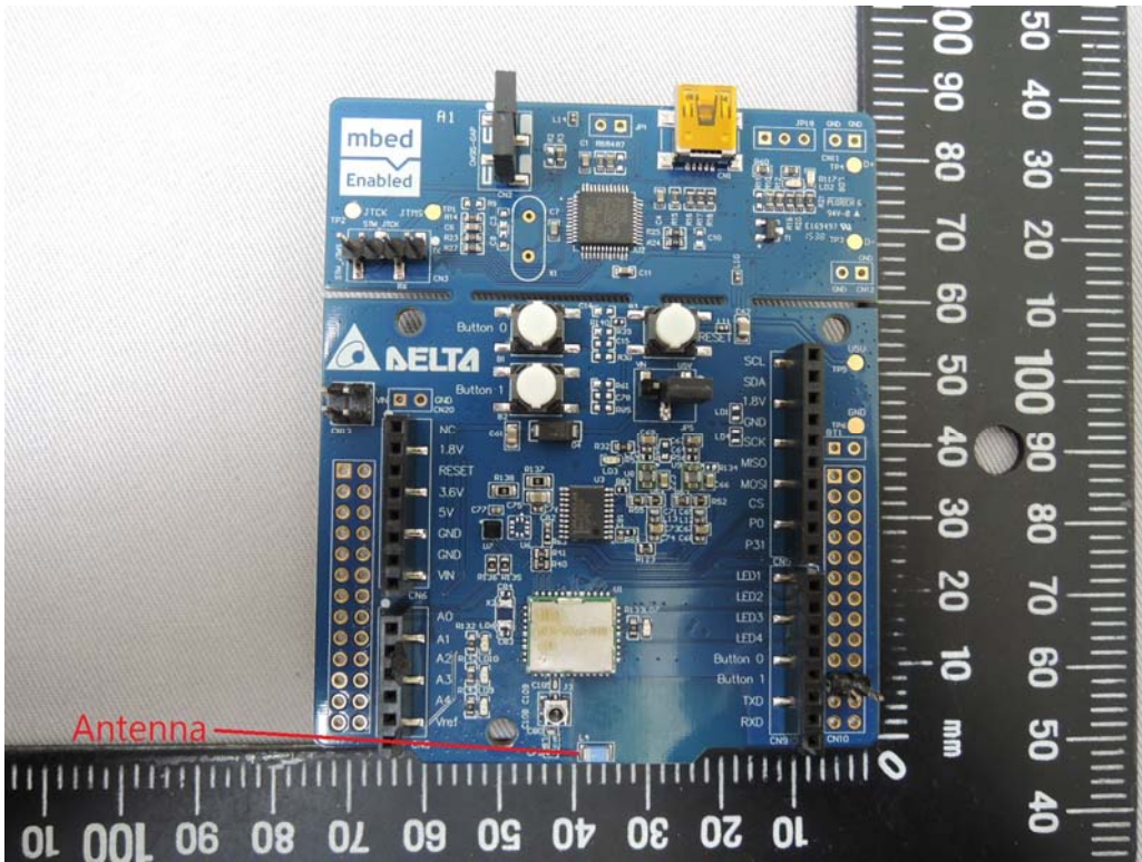
BT Antenna
