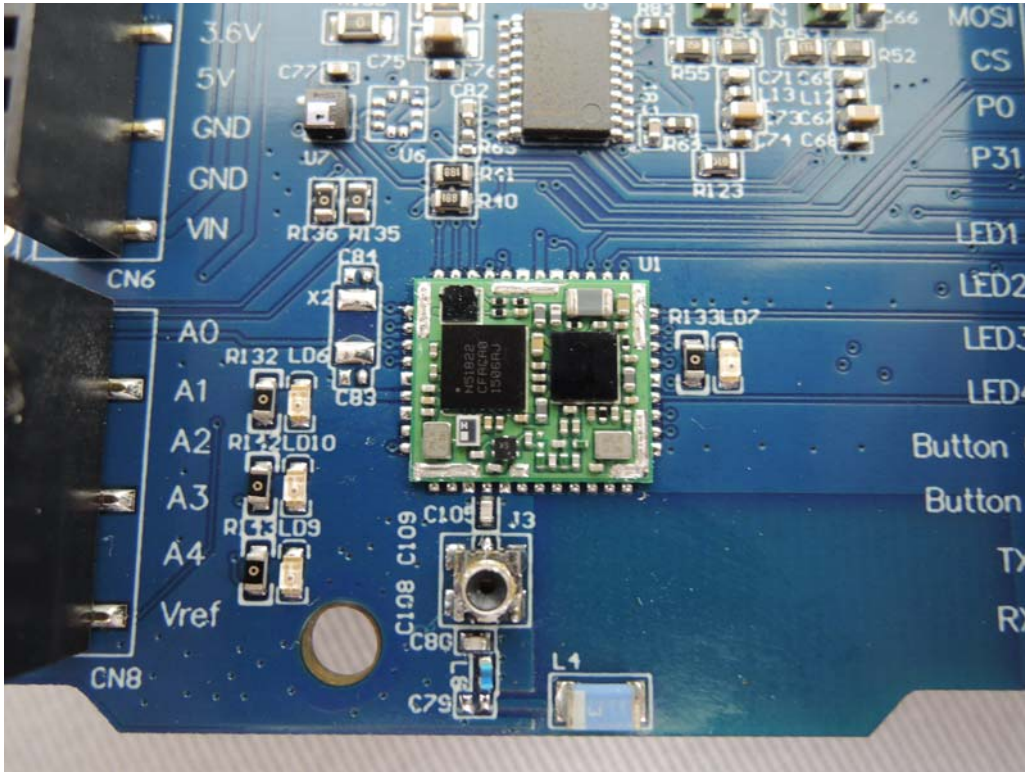
BT Antenna
