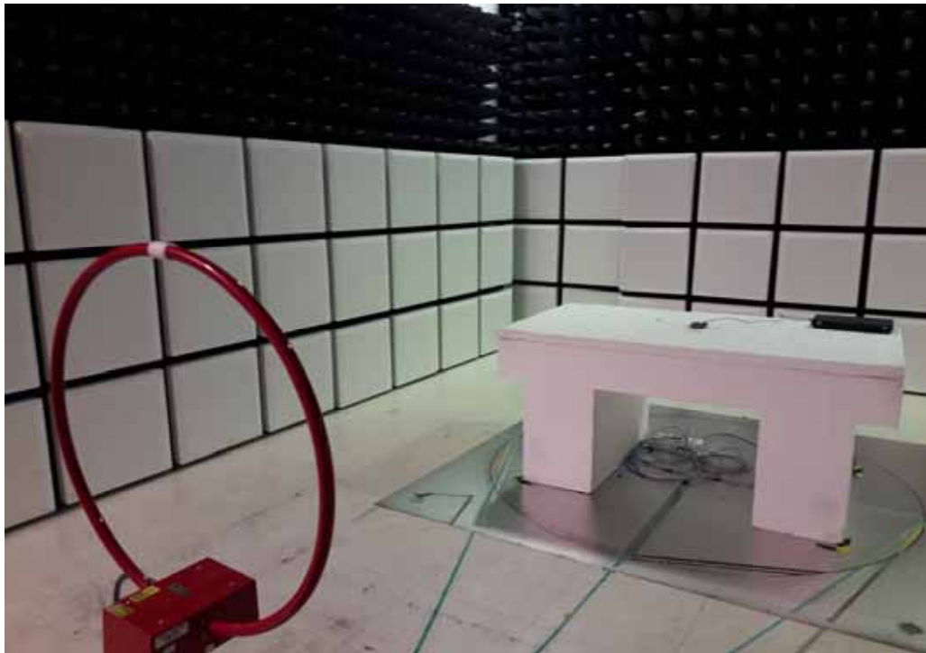
Radiated Emission Set up Photos (Below 1GHz)
