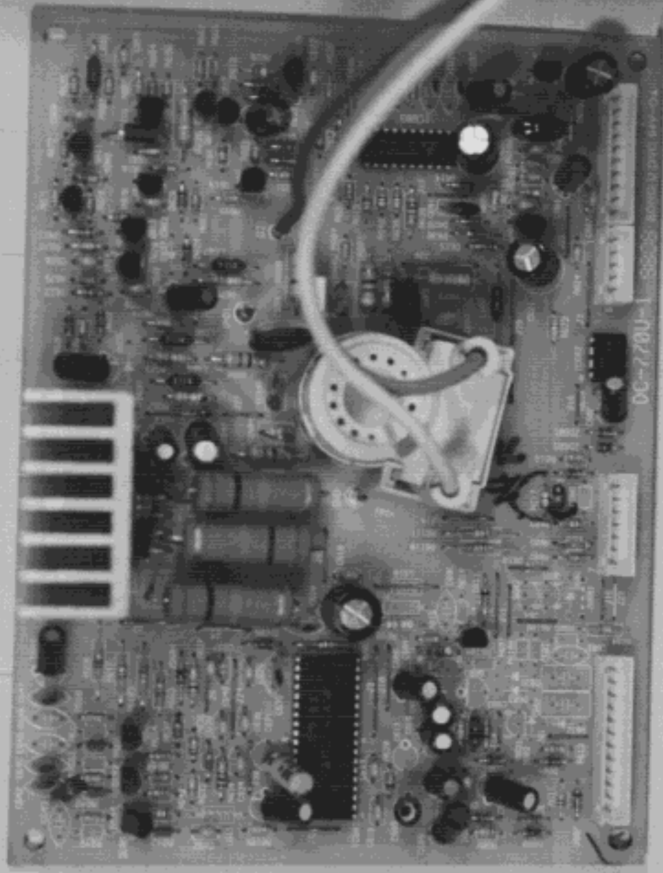
FCC ID: H79DC-770 Front side of CRT board
