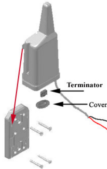
Figure 2: Wall Mounting
