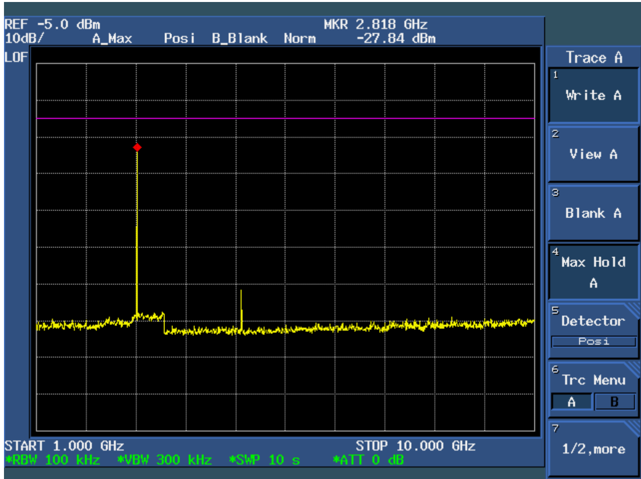
Plot # 44: Spurious Emissions Conducted @ 851 – 869 MHz Output with 3 RF Input signals Fc: 869 MHz, Fc - 25 kHz, & Fc – 12.5 kHz
