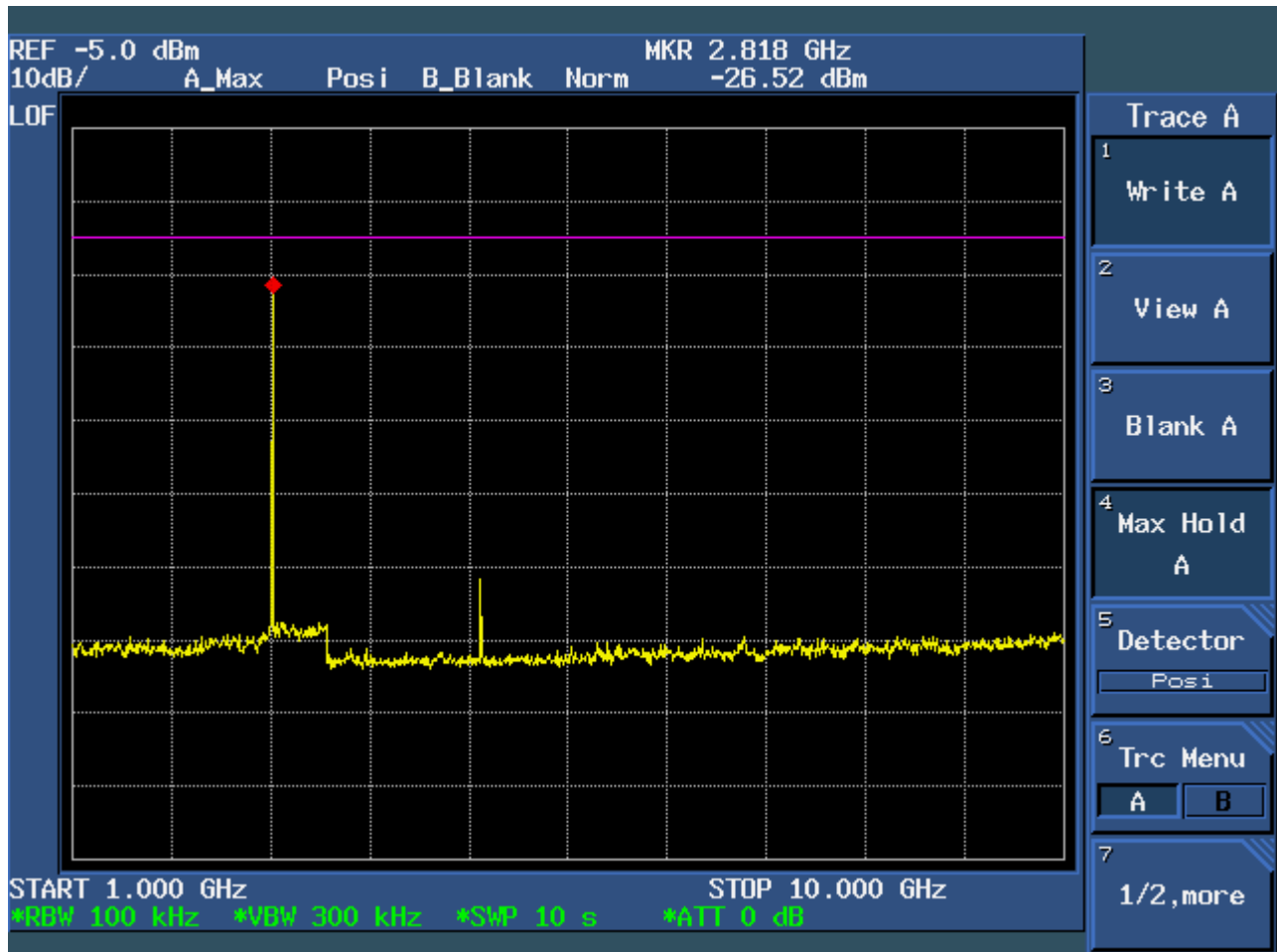
Plot # 42: Spurious Emissions Conducted @ 851 – 869 MHz Output with 2 RF Input signals Fc: 869 MHz, Fc - 12.5 kHz
