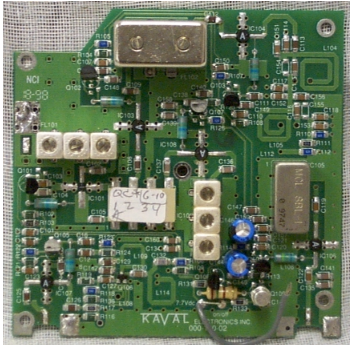
Photograph 14. Top View of Front End Module Board (Shields Removed)
