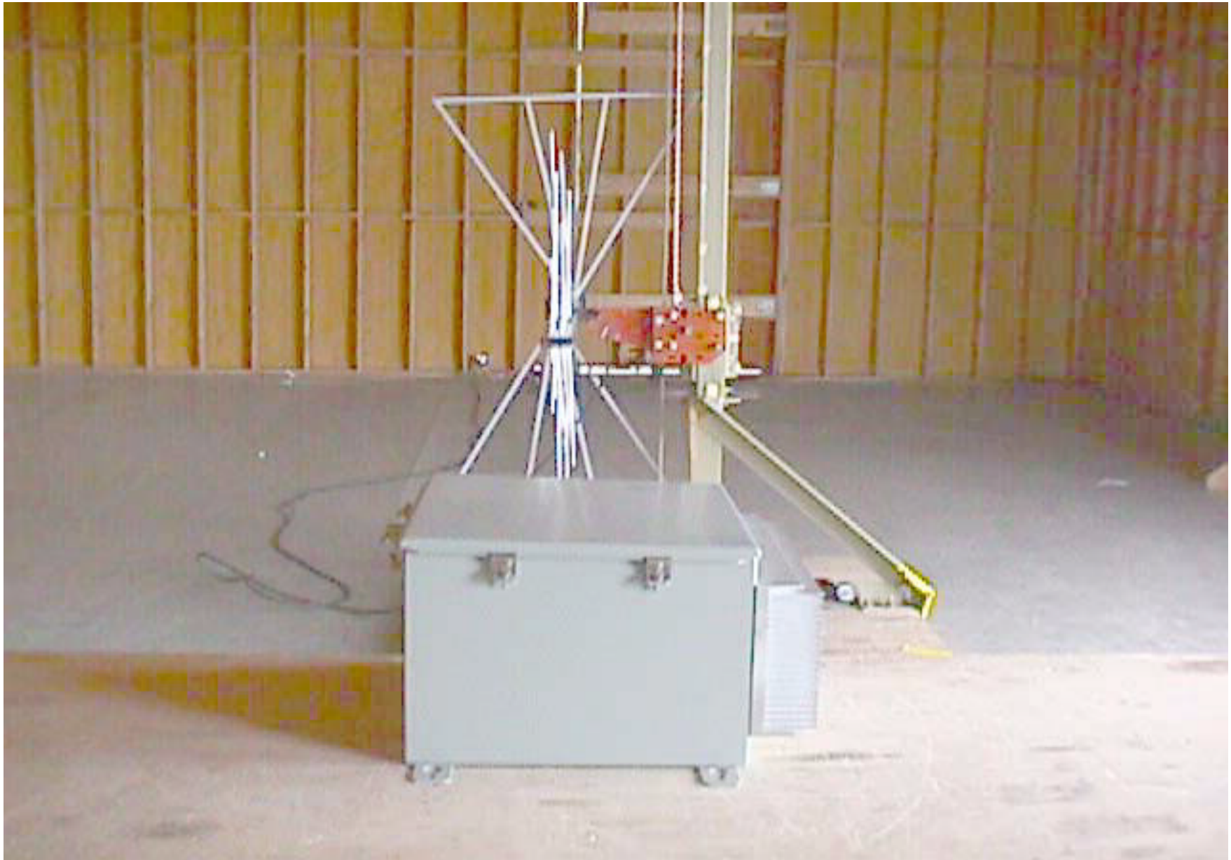
EXHIBIT 10 - PHOTOGRAPHS OF TEST SETUP FOR RADIATED EMISSIONS PHOTO #1 OF 2
