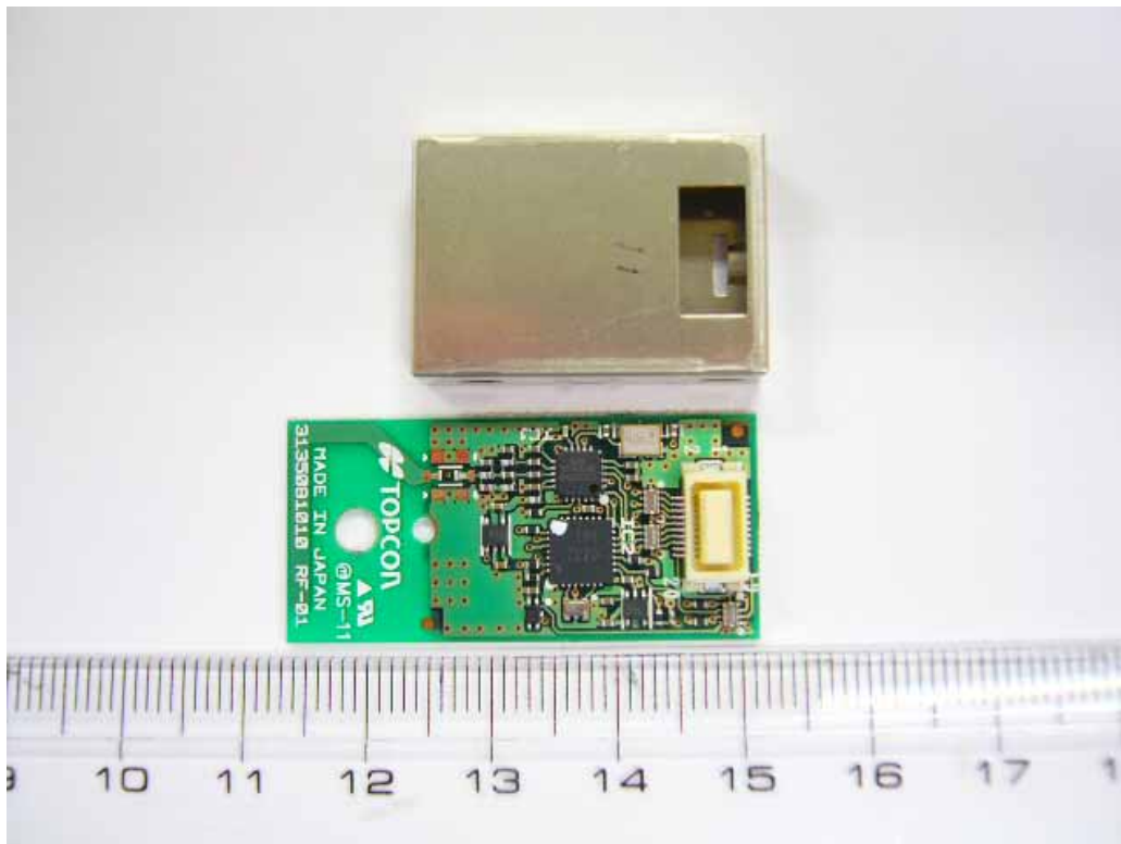
Top Case and inside PCB
