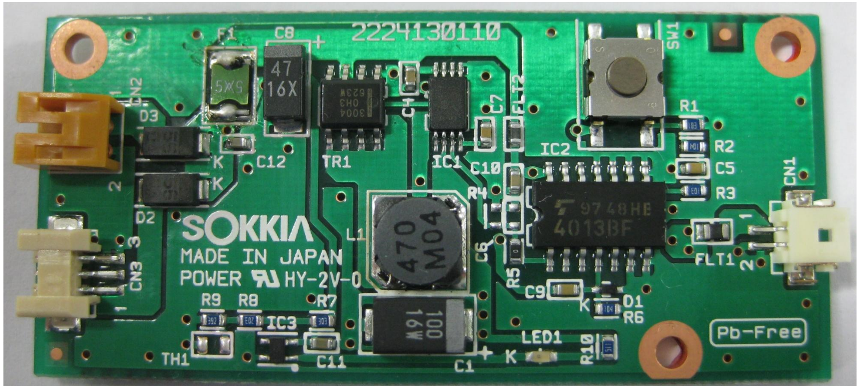
Power board upper side
