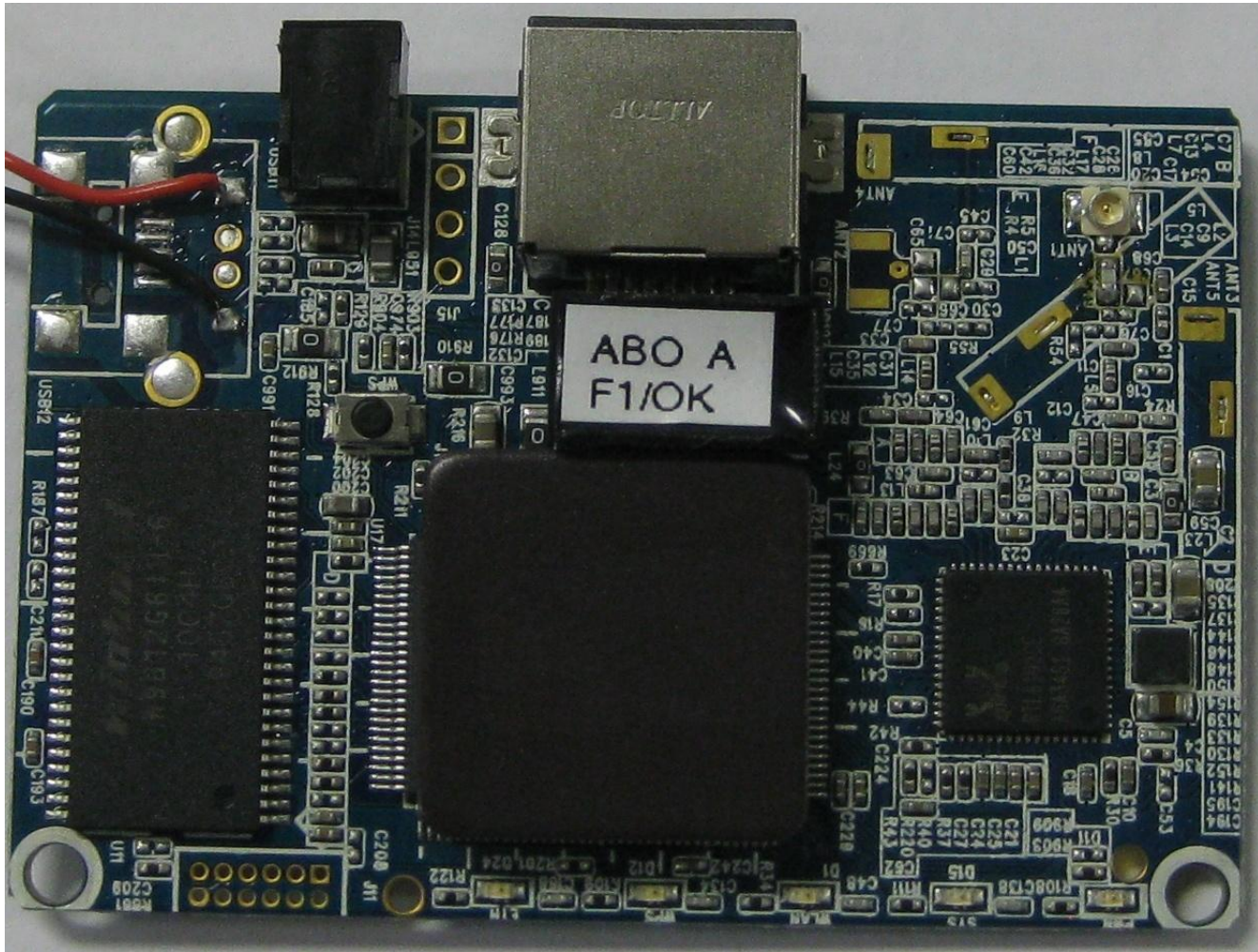
WLAN board top side
