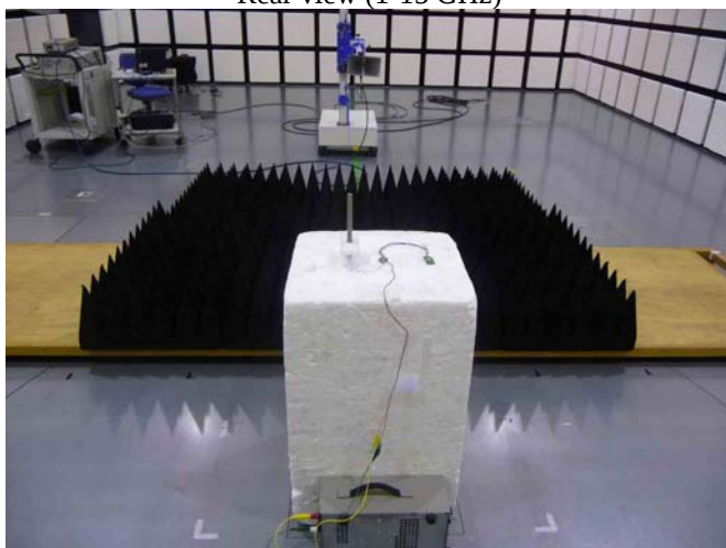
Rear view (15-18 GHz)
