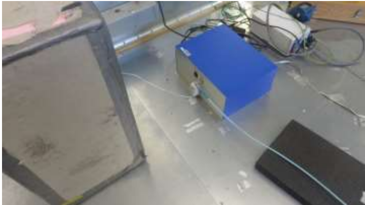
AC Mains Conducted emissions setup
