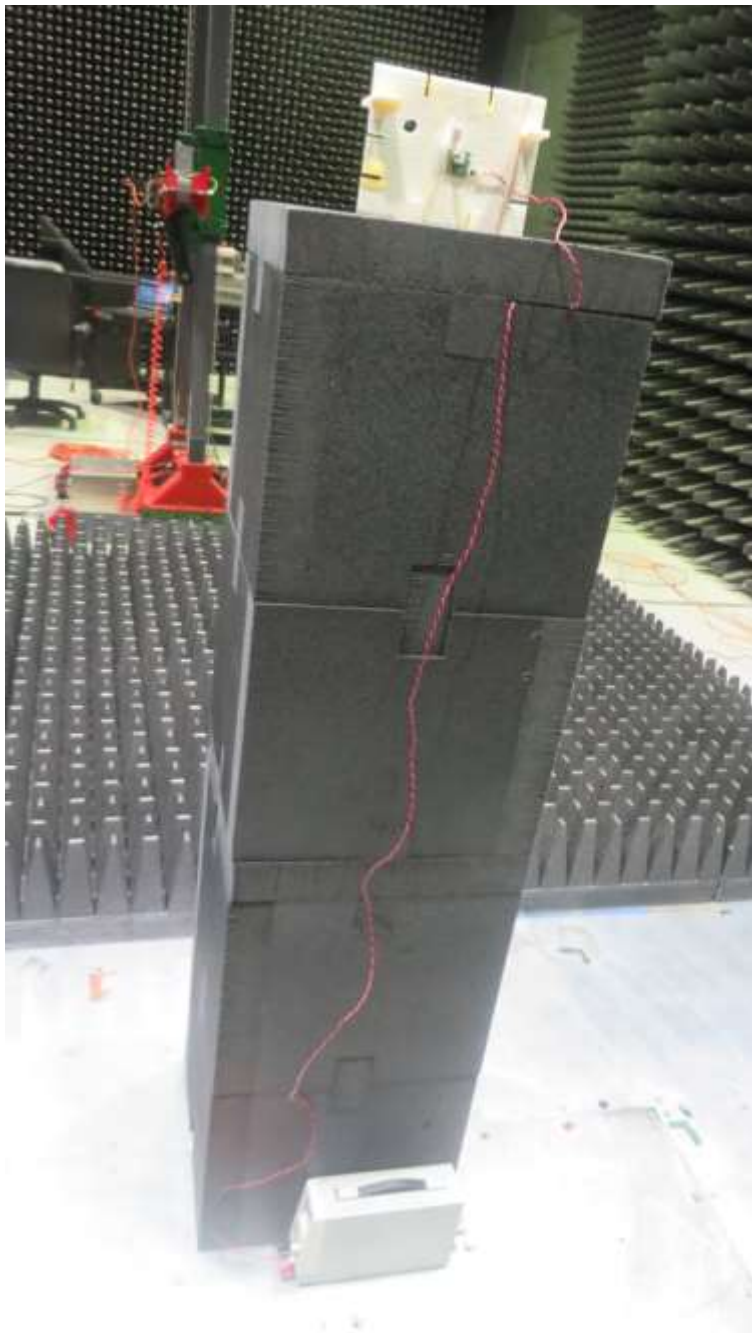
Above 1 GHZ setup
