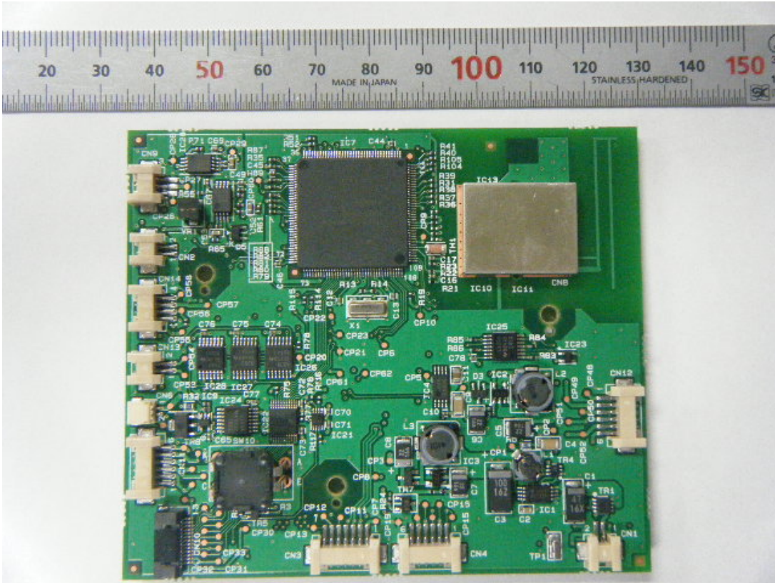
PCB Topside View(with Shield Case)
