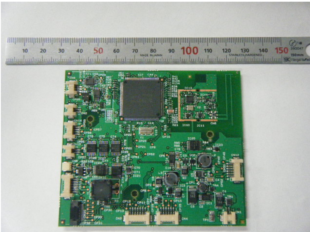
PCB Topside View
