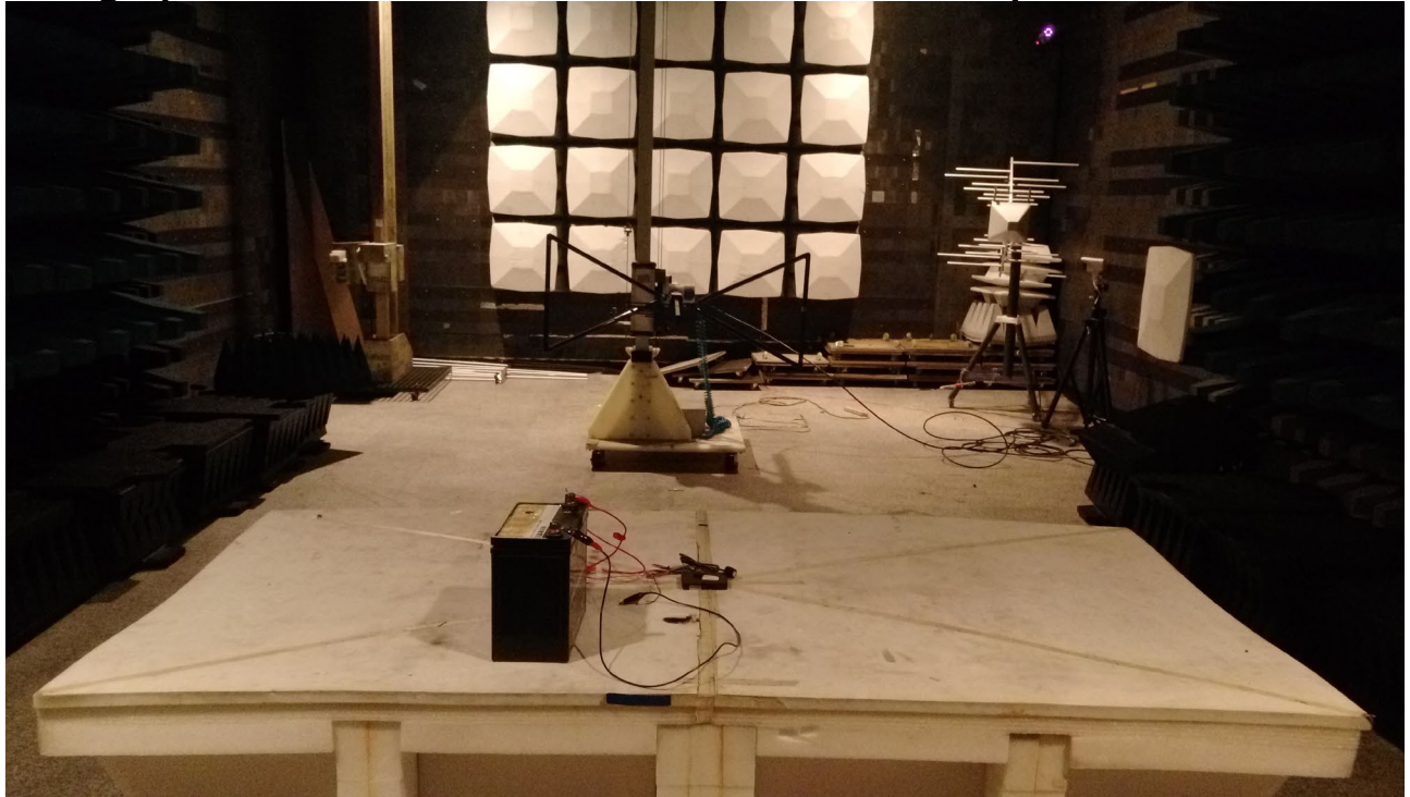
Photograph – Radiated Emission Below 1G Test Setup
