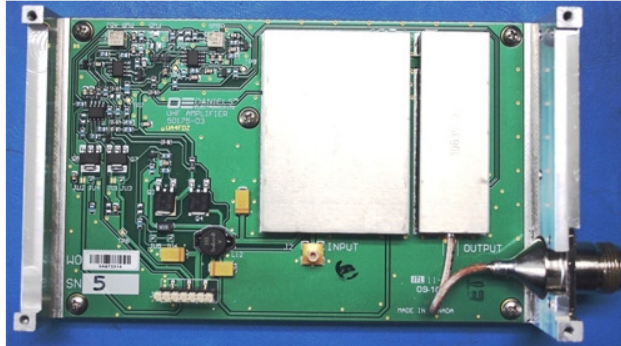
900MHz Amplifier Board with Heat Sink
