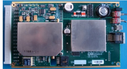
Main Board Top View
