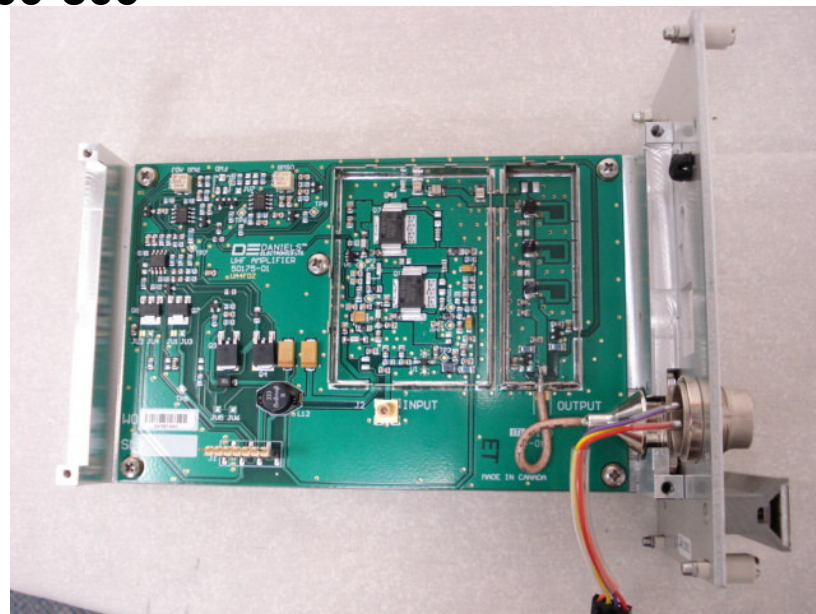
UHF Amplifier, shields removed
