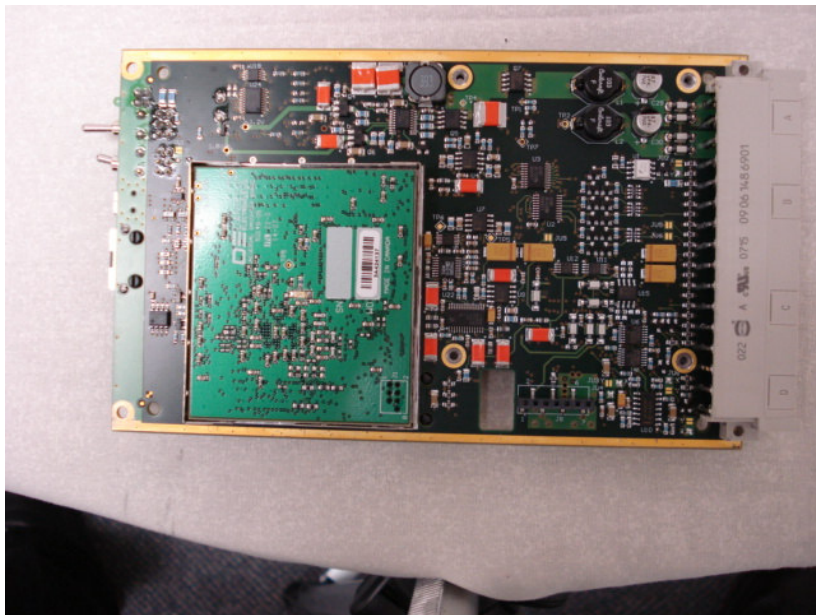
Transmitter Main Board, Bottom View, UDB Shield removed
