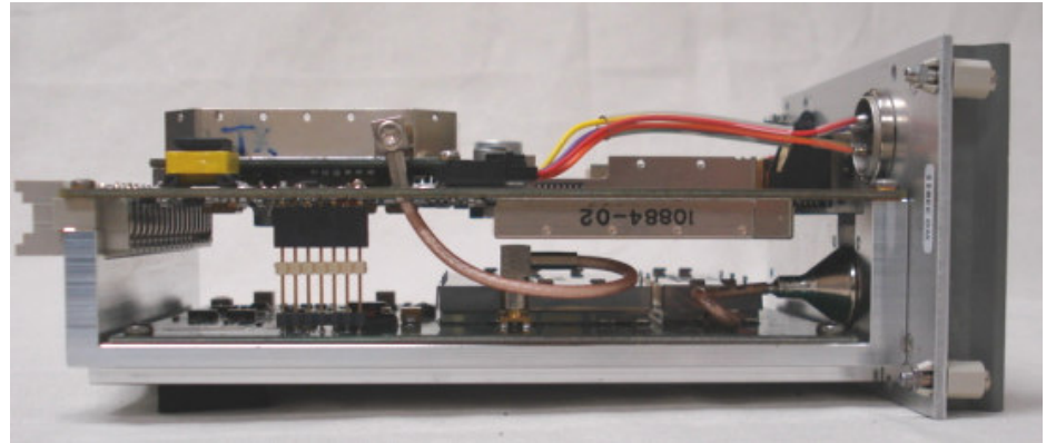
Transmitter, Bottom Side View showing UHF Amp and Transmitter Main Board
