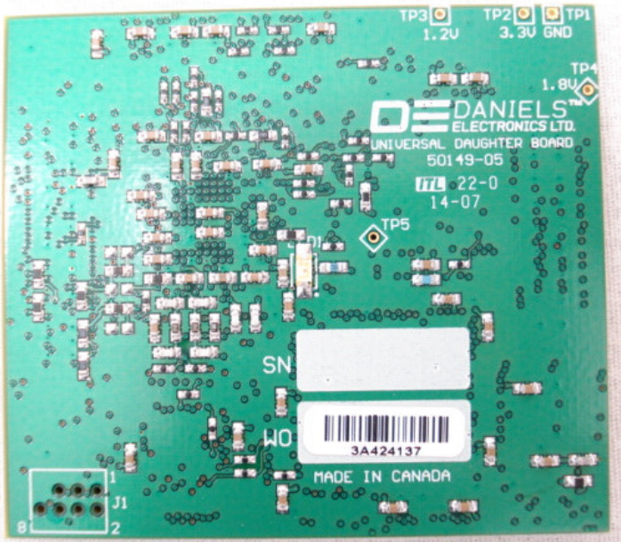
Universal Daughter Board – Bottom View
