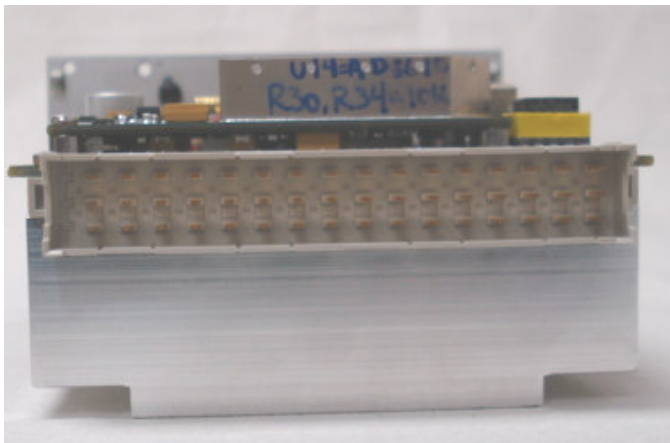
Rear Connector End View
