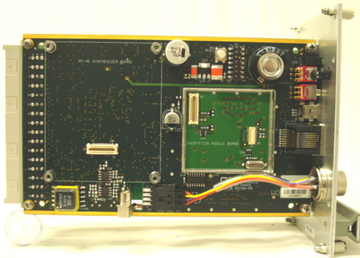
Transmitter Main Board, UHF PA & Encryption Module Shield Removed
