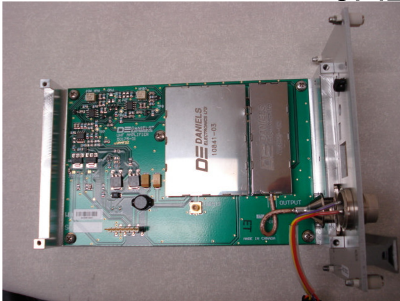
UHF Amplifier, shields in place
