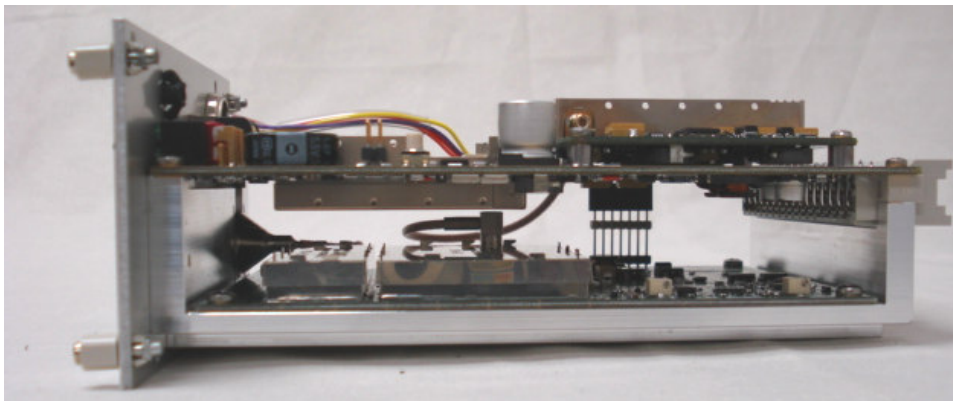
Transmitter, Top Side View showing UHF Amp and Transmitter Main Board
