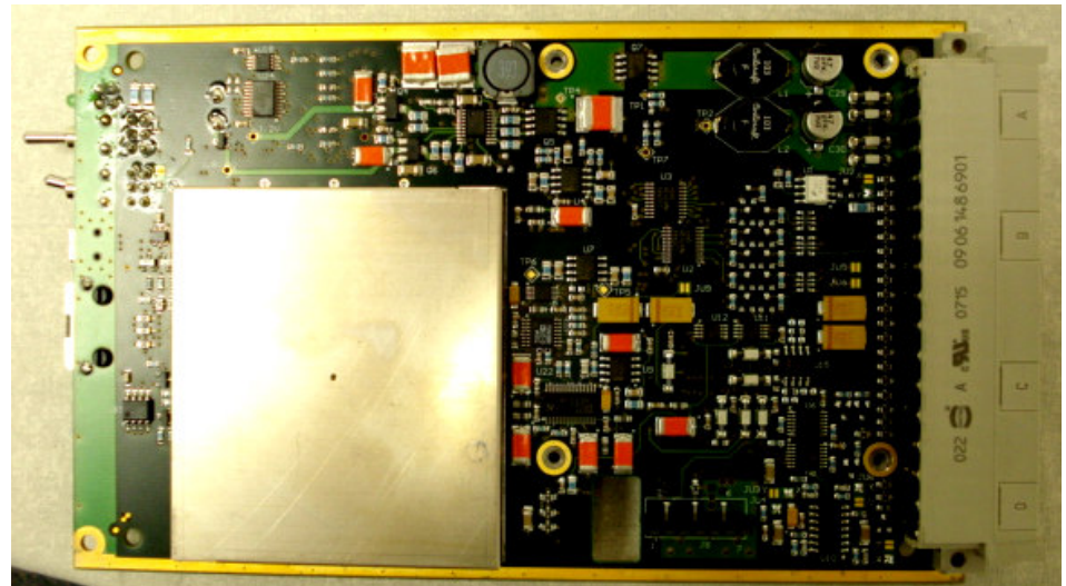
Transmitter Main Board, UDB Shield in place
