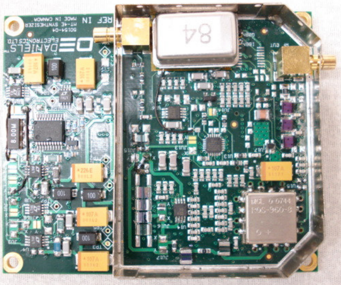
Synthesizer, top view, shield lid removed
