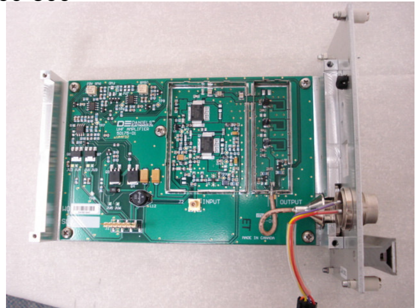
UHF Amplifier, shields removed
