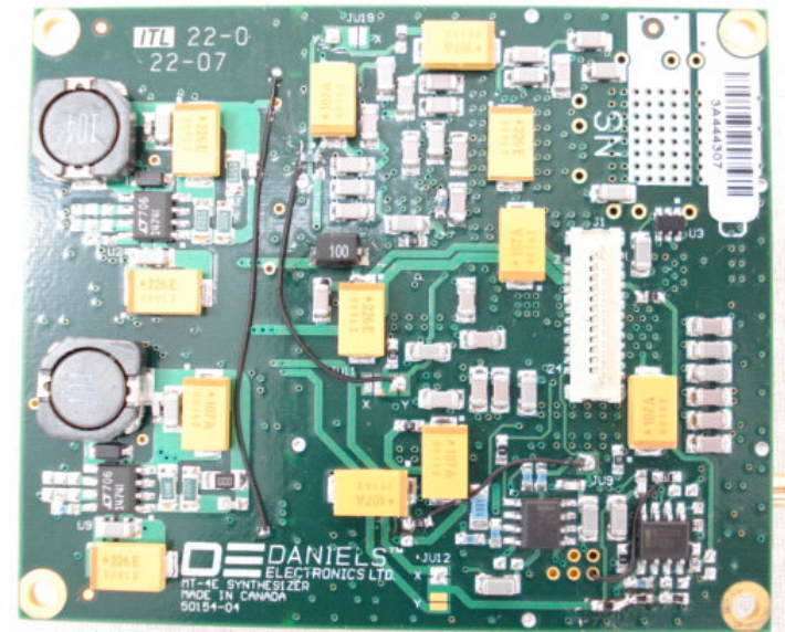
Synthesizer, bottom view
