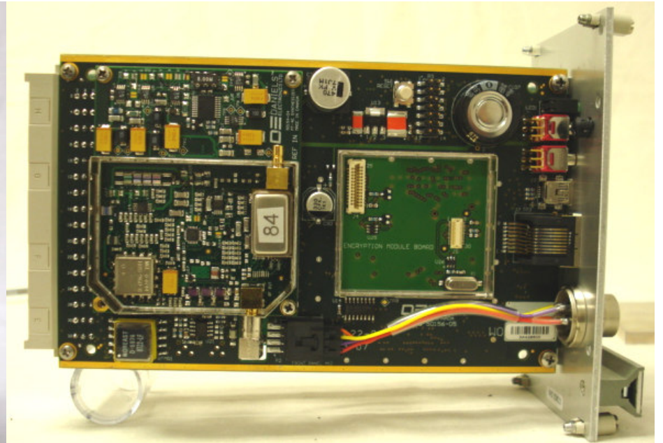
Transmitter Main Board, Synthesizer and Encryption module Shields removed
