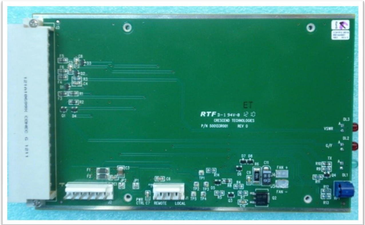
1 – Alarm Board Front
