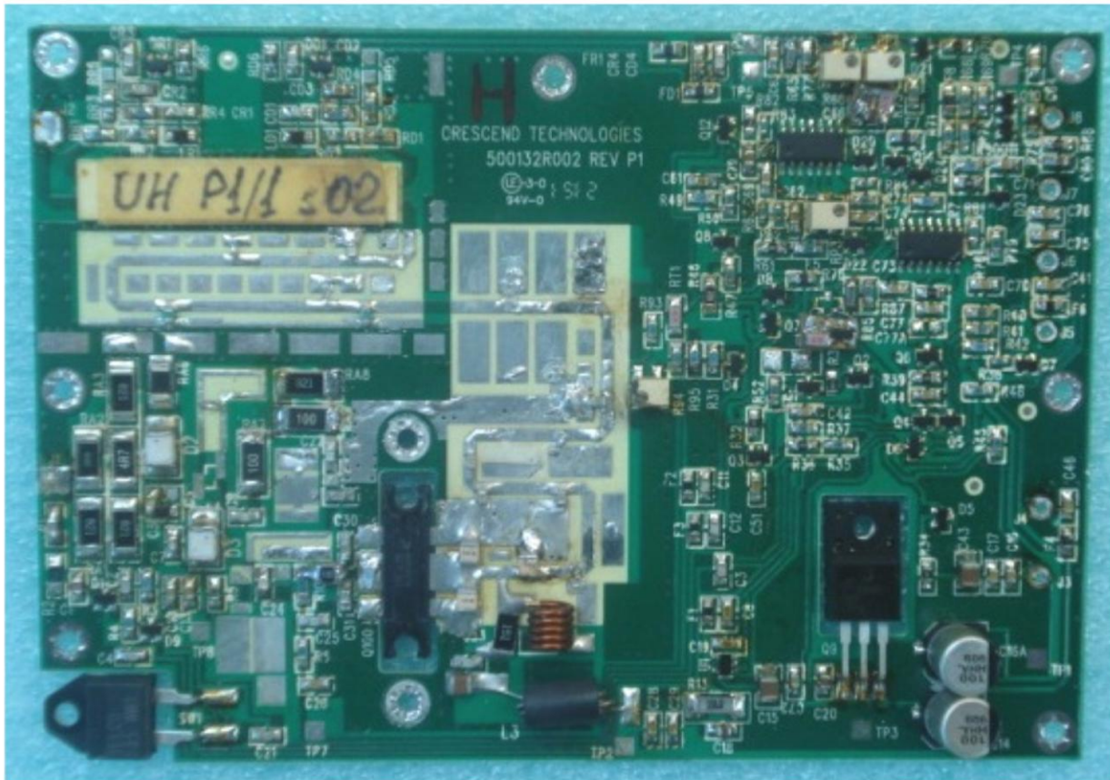
3 – AMP Board Front
