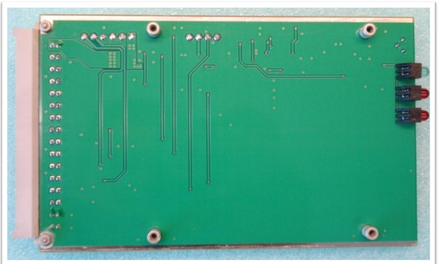
2 – Alarm Board Back
