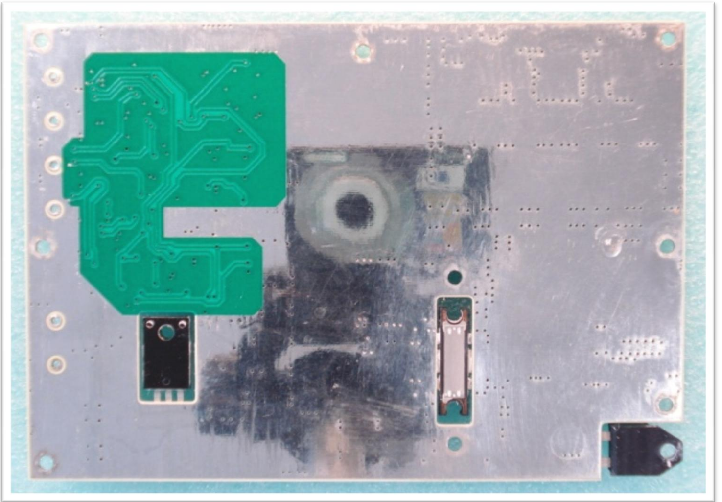
4 – AMP Board Back
