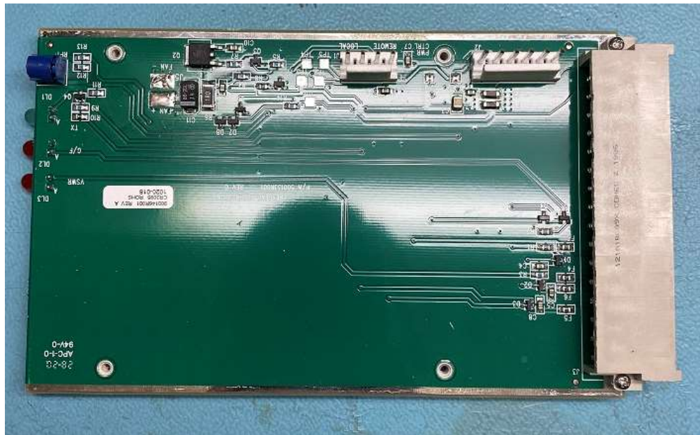
1 – DC Connector Board Front (replaces 1 – Alarm Board Front)
