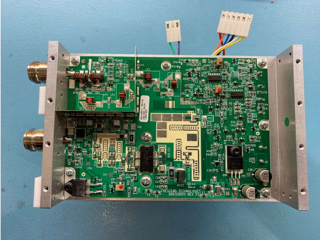
3 – Main Board Front (replaces 4 – Amp Board Front)
