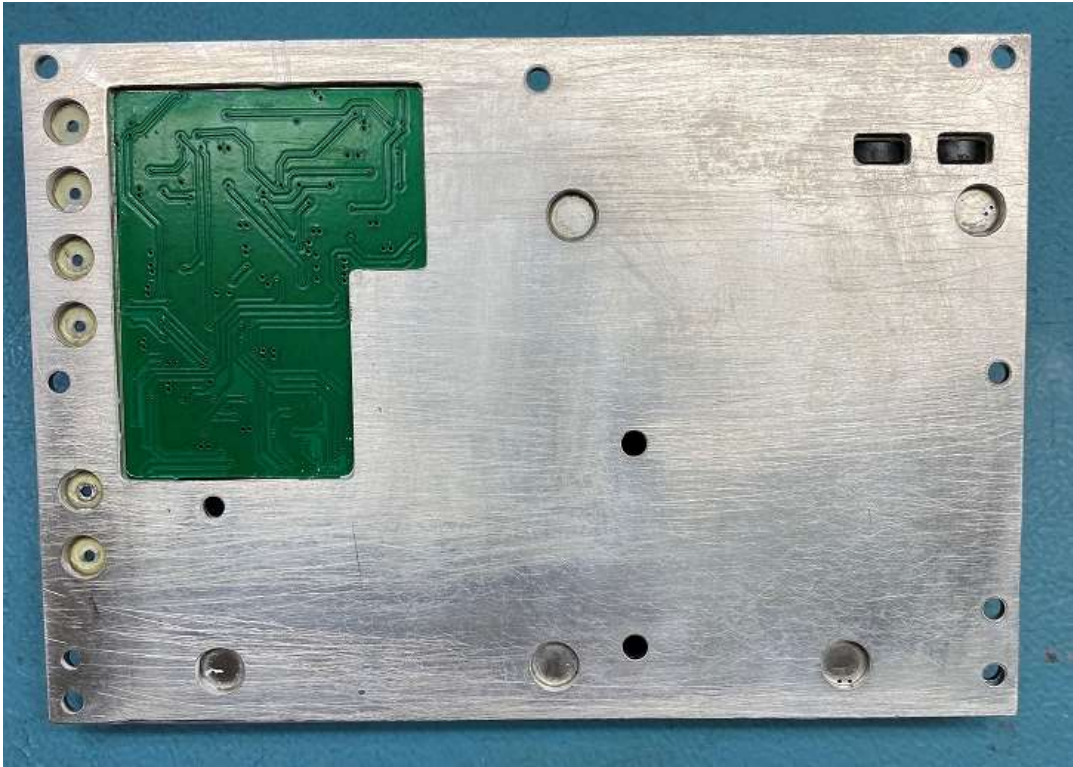
4 – Main Board Back (replaces 5 – Amp Board Back)
