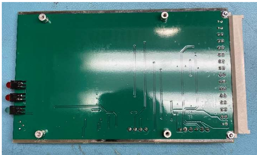
2 – DC Connector Board Back (replaces 2 – Alarm Board Back)
