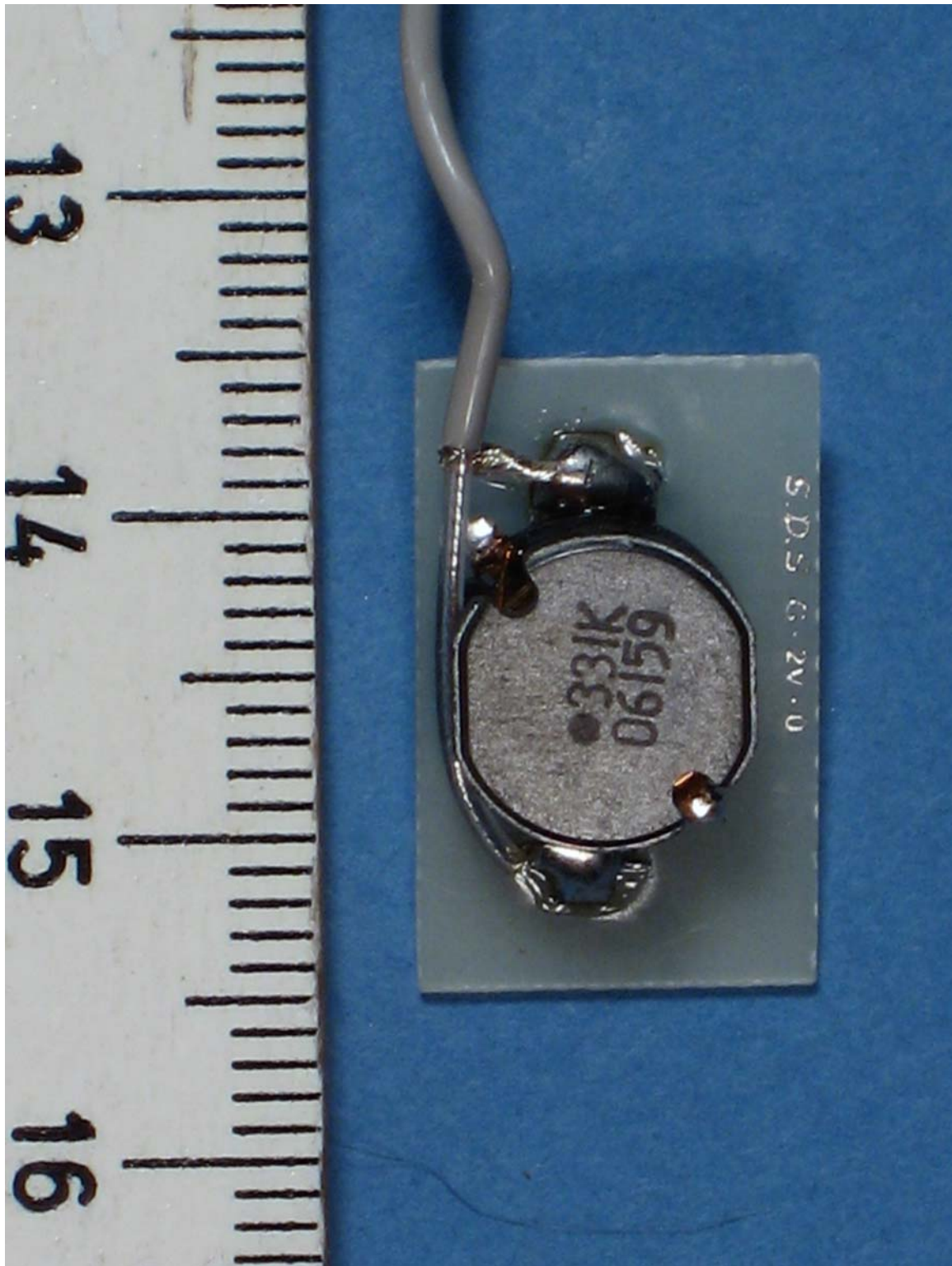
Photograph 7: - Steam Trap Management System, model TM6, RFID antenna, top view
