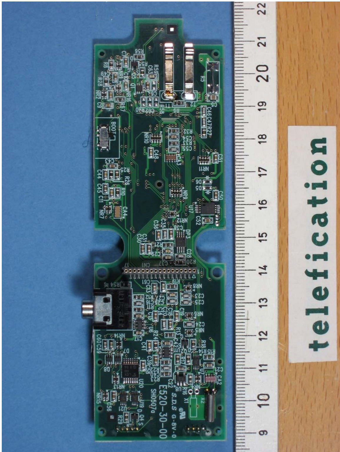
Photograph 10: - Steam Trap Management System, model TM6, main PCB, rear view
