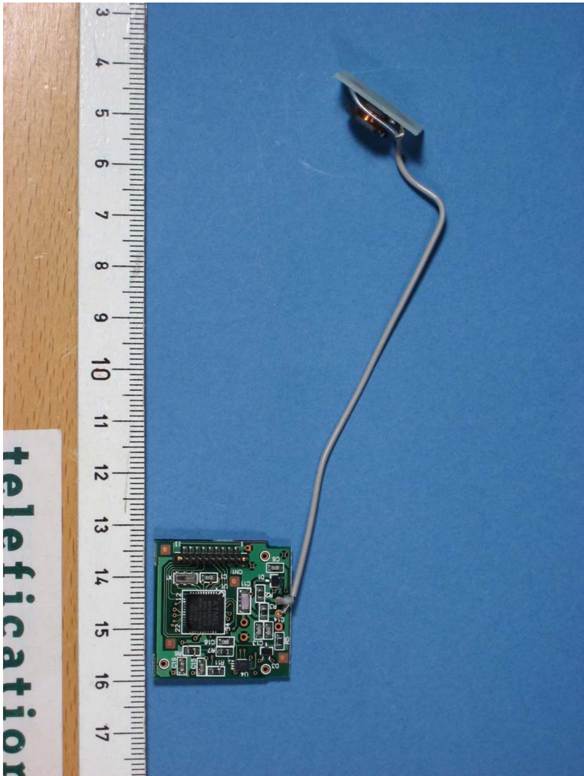
Photograph 6: - Steam Trap Management System, model TM6, RFID PCB incl. antenna
