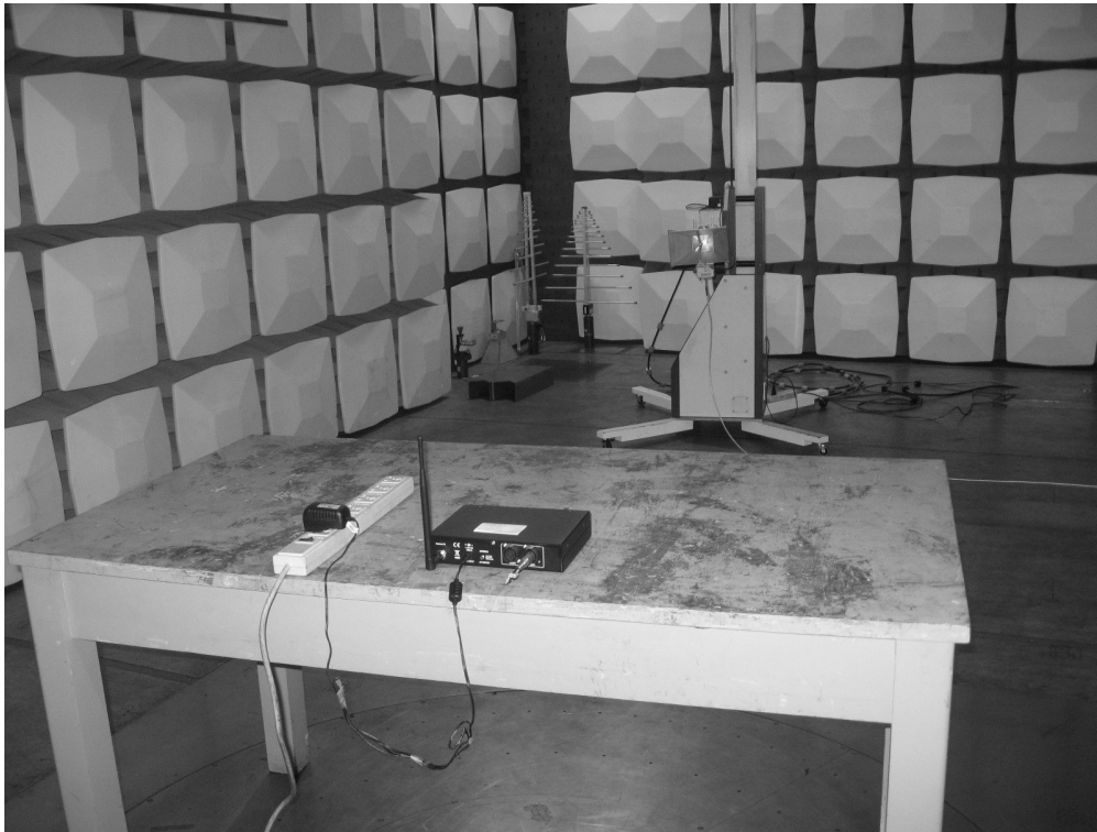
Substitute antenna
