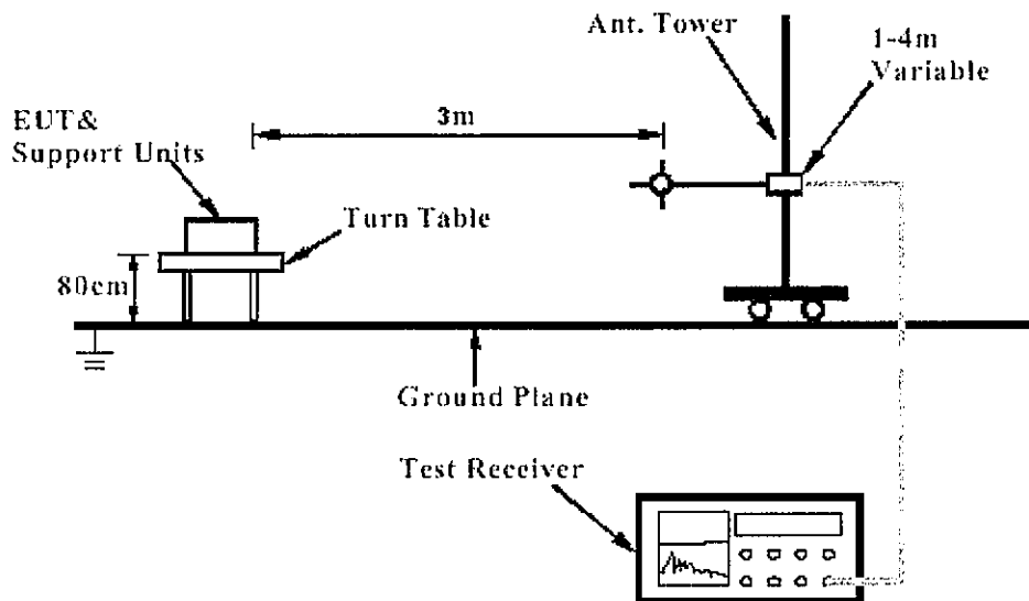
Diagram 2 of Measurement Equipment Configuration for Substitution Method
