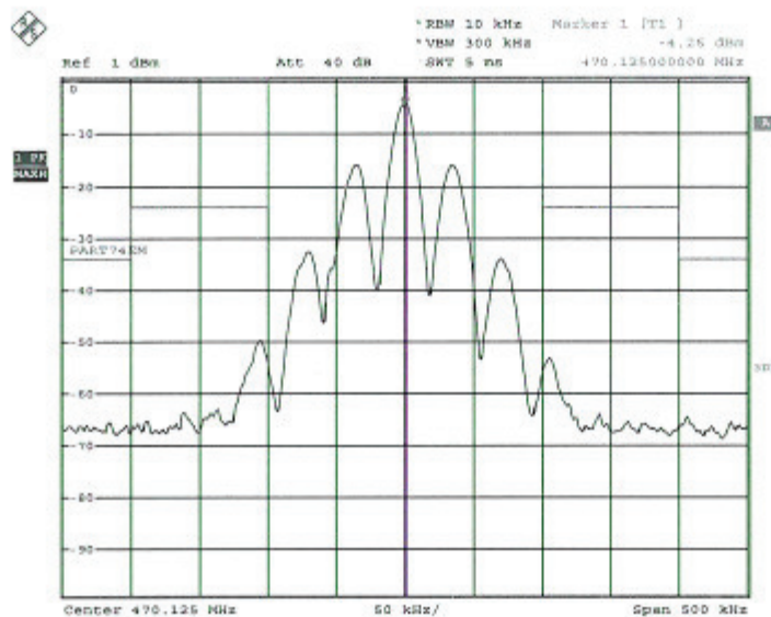
Figure 17: Emission Mask (U-899P, Low CH)
