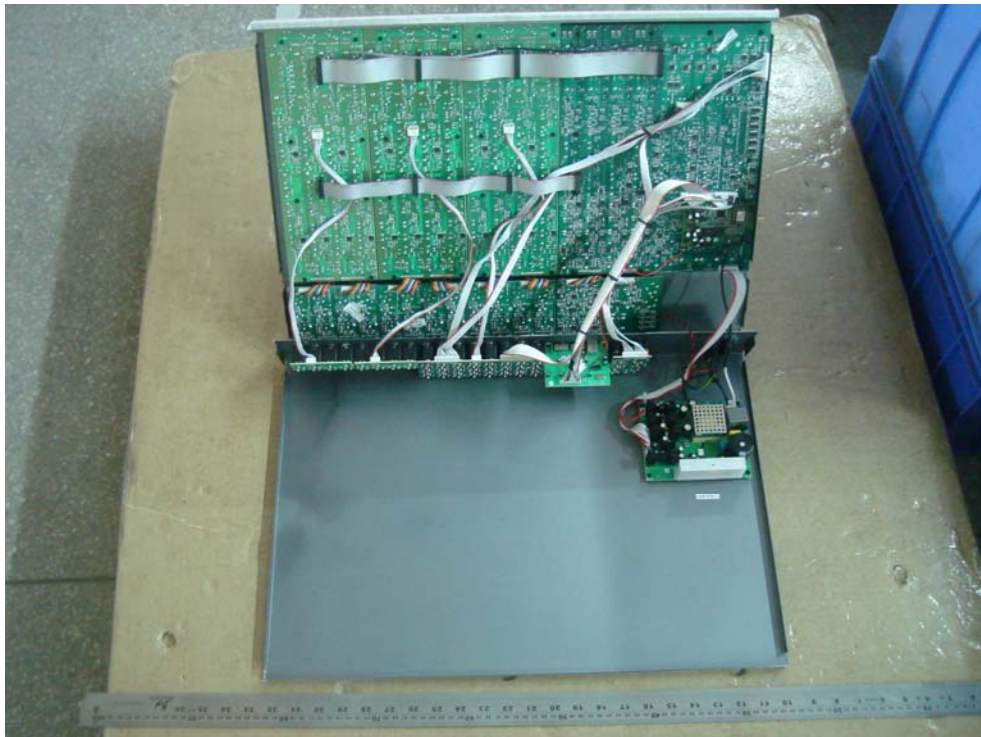
LYNX-MIX204 USB Internal Photo
