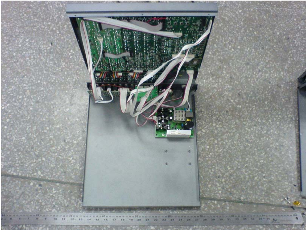
LYNX-MIX124 USB Internal Photo
