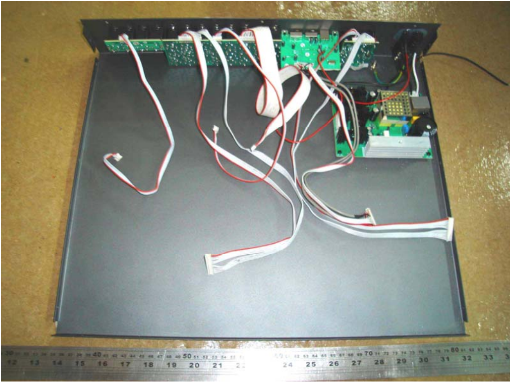
LYNX-MIX164 USB Internal Photo
