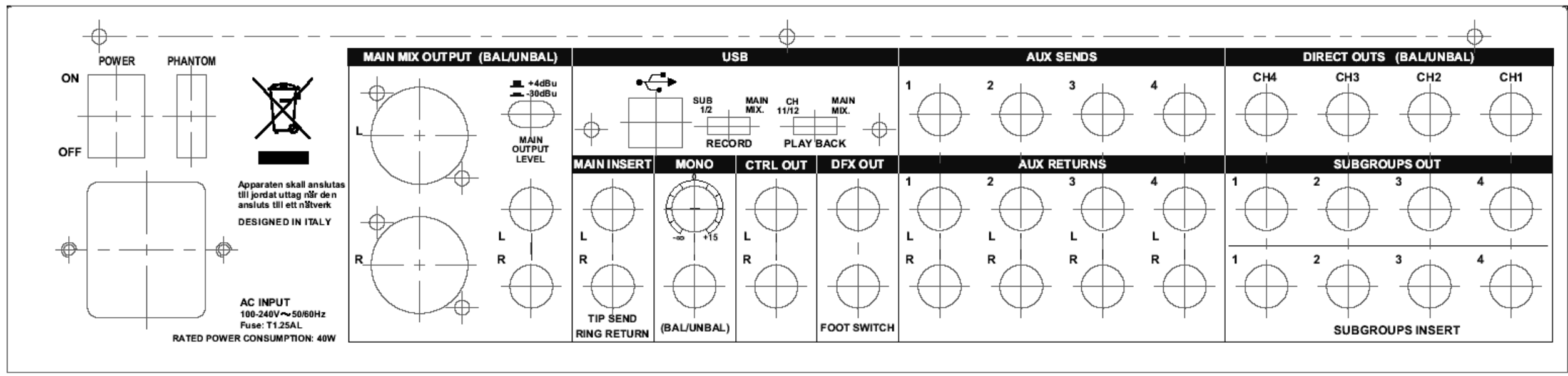
LYNX-MIX124 USB
