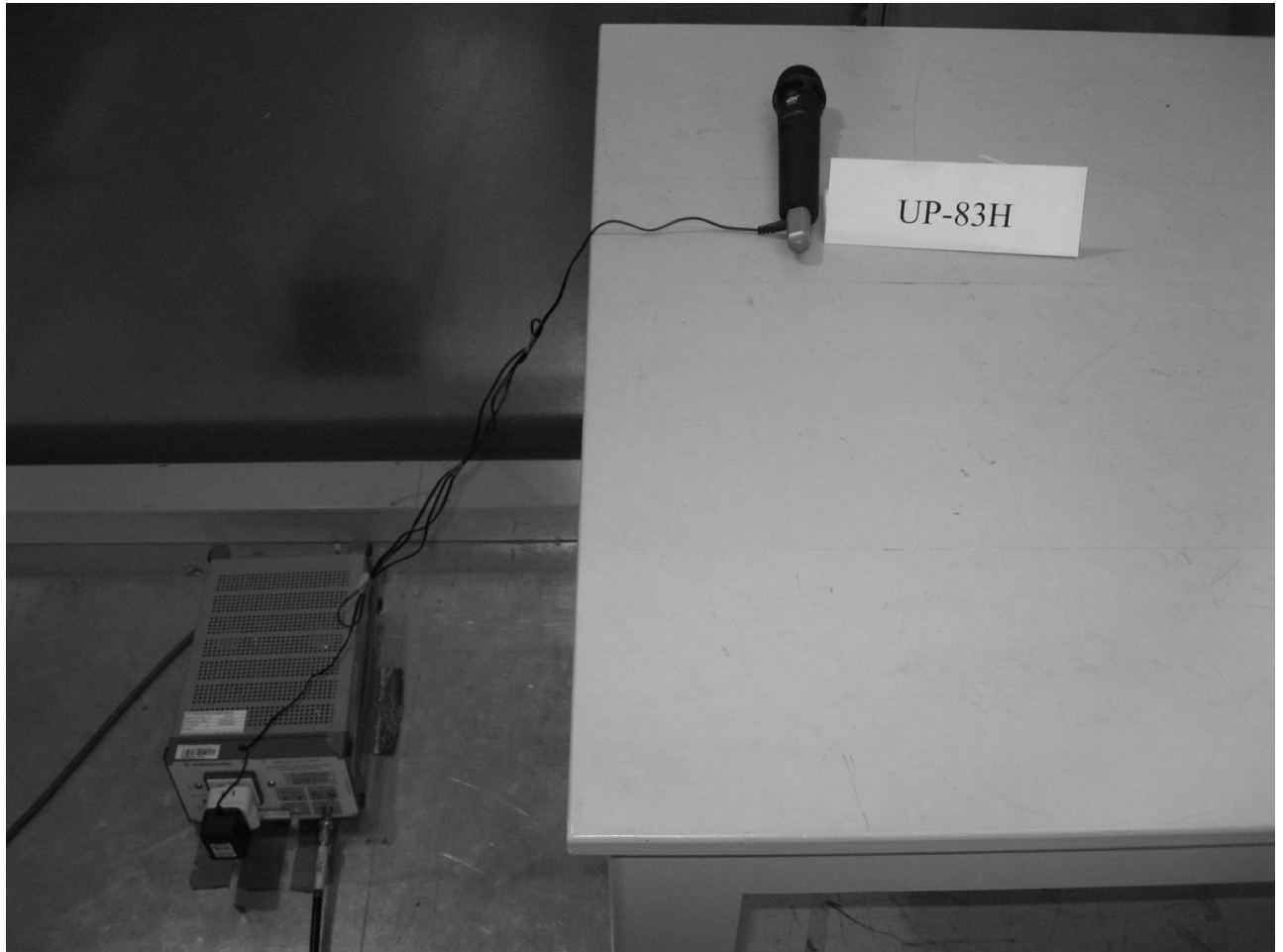
Photograph 3: Set-up for Conducted Emission of AC mains
