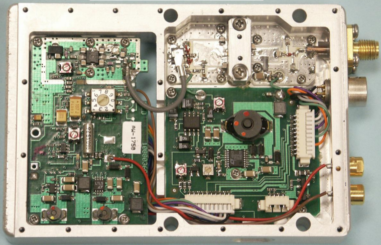
Video/RF Driver, Pwr Supply, Matching Networks
