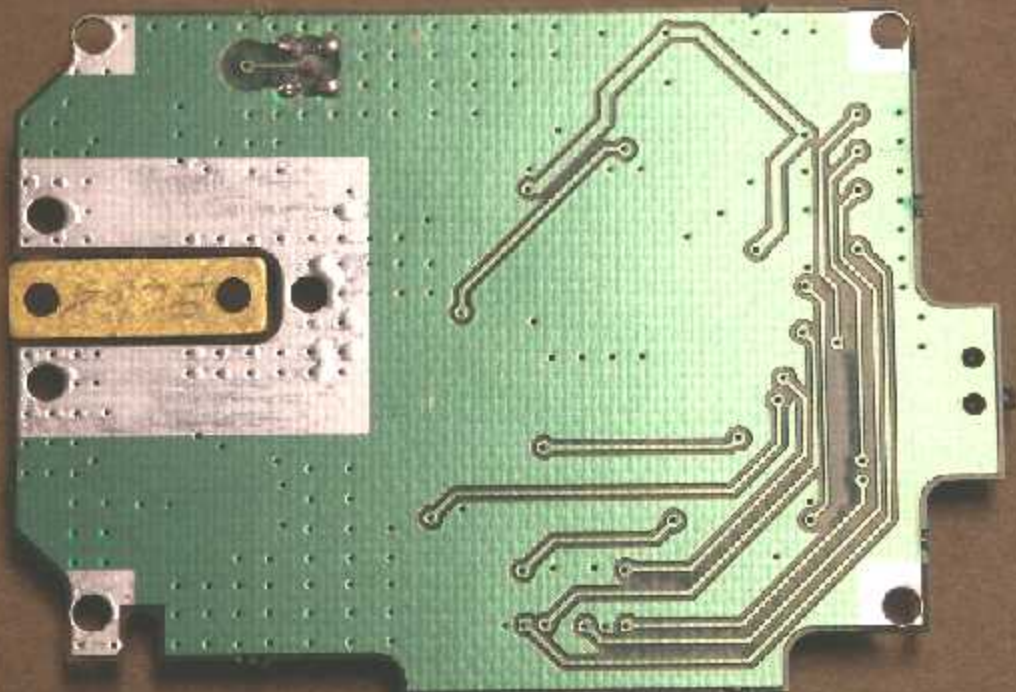
2 Watt Amplifier PCB / back
