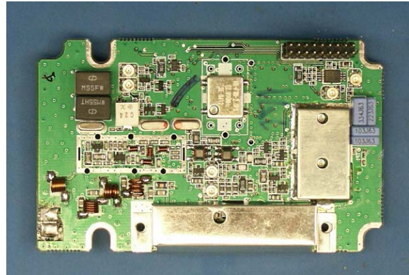
Maxon Transceiver RF CCA, Top View With Shields
