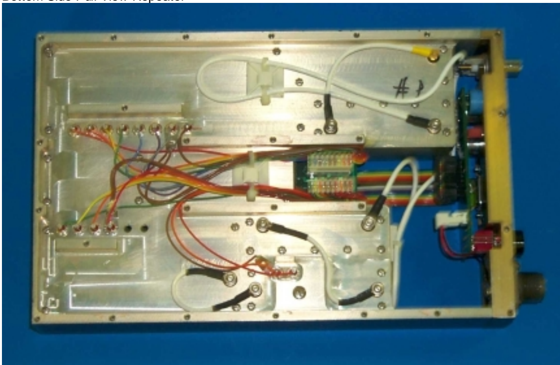
Bottom Side Full View Repeater
