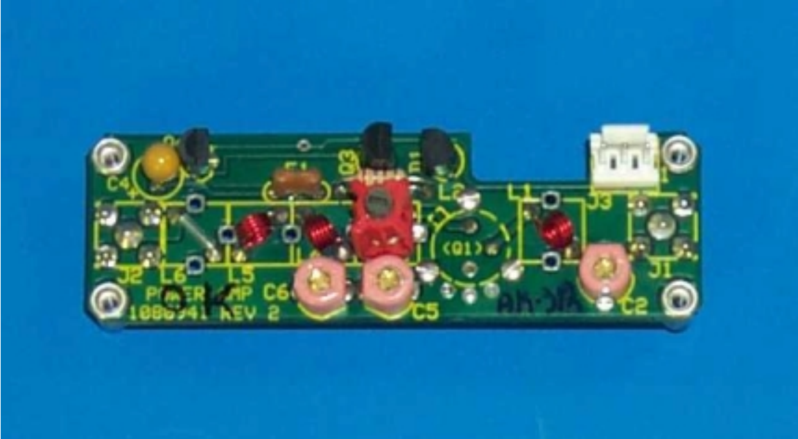
Top Side Repeater Power Amplifier
