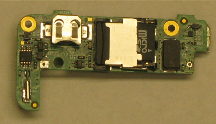
Digital Board Bottom View
