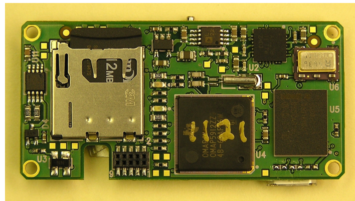
Digital Board Top View
