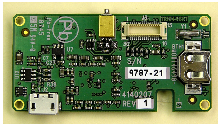
RF Board Bottom View
