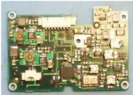
RF board, top view
