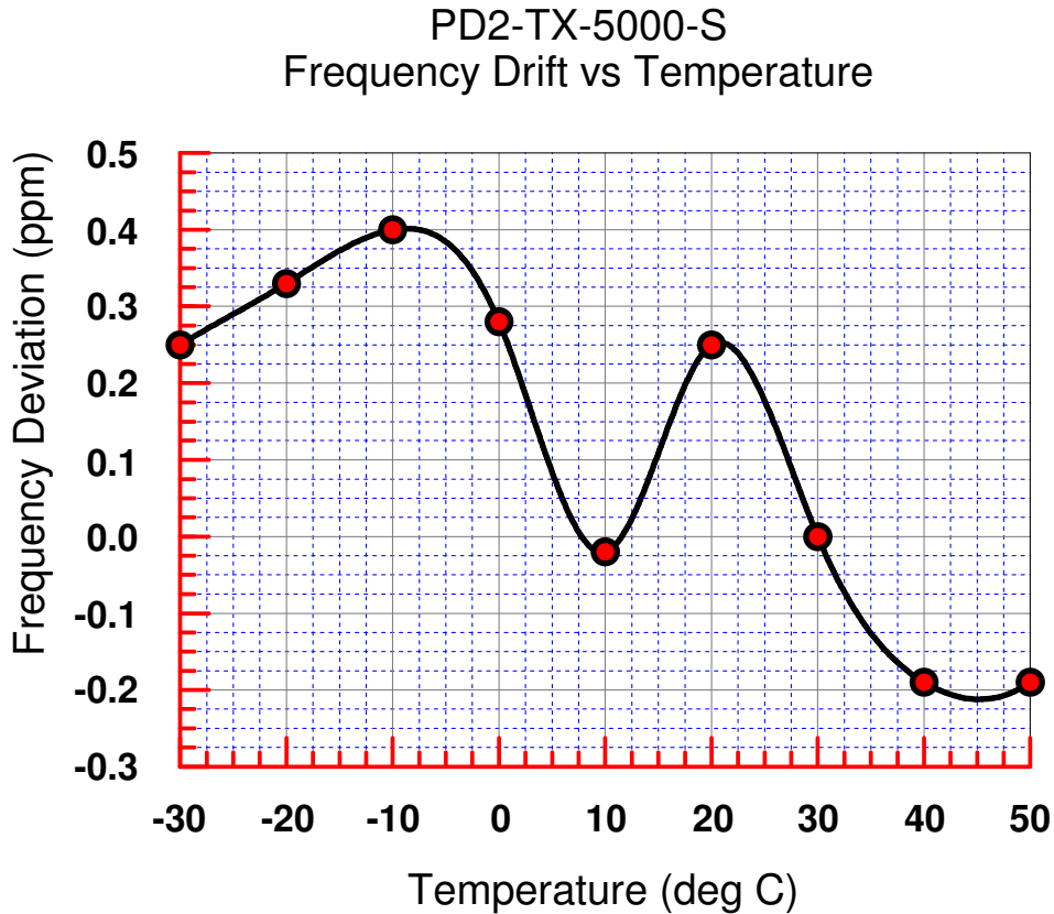
Figure 17b - Frequency Deviation as a Function of Temperature (Pursuant to FCC Requirement 2.1055a)
