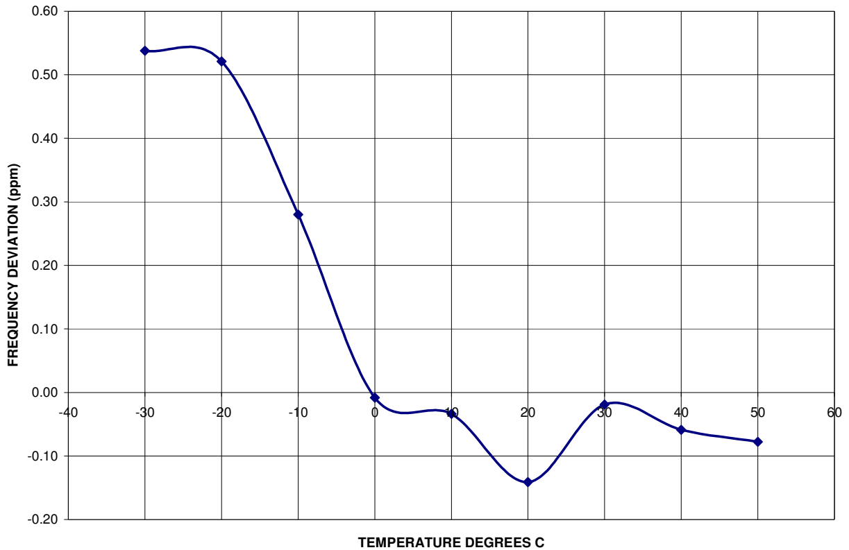
PD2-TX-1000-SV: FREQUENCY DEVIATION vs. TEMPERATURE
