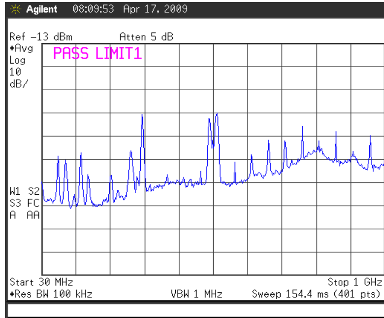
Fig. 10a Spurious Emissions Compliance 30MHz – 1GHz TX Mode = DVB-T Emission: 8M0W7D
