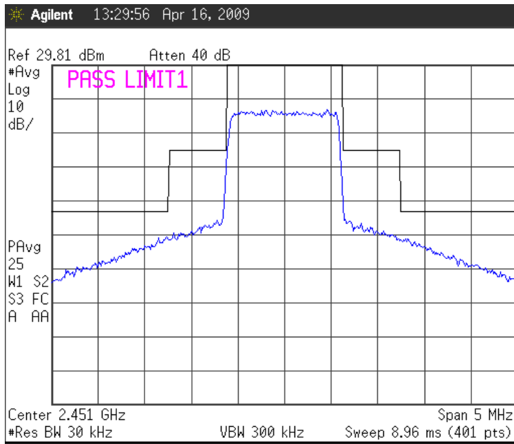
Fig. 12a Emission Mask Compliance TX Mode = DOMO-N Emission: 1M3W7D Lower Band Edge
