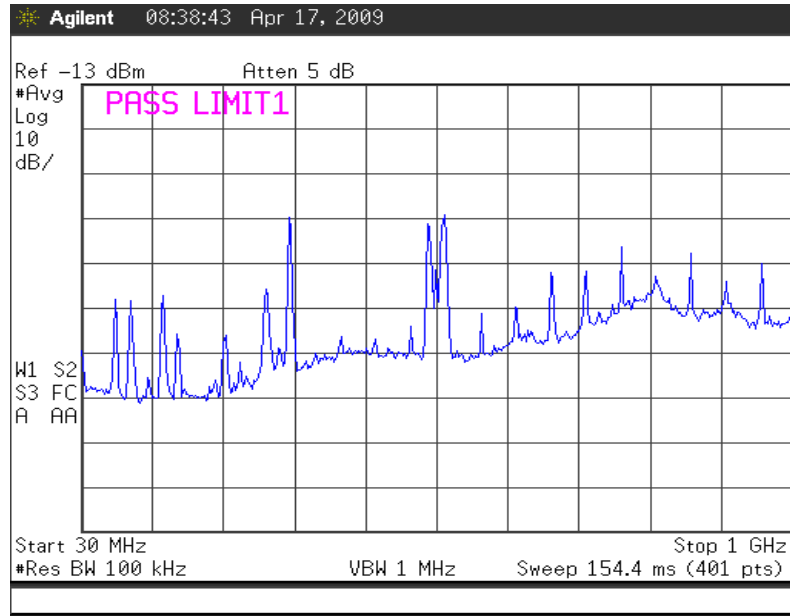
Fig. 8a Spurious Emissions Compliance 30MHz – 1GHz TX Mode = DVB-T Emission: 6M0W7D
