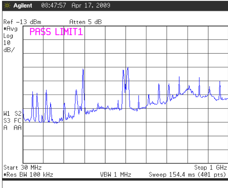
Fig. 9a Spurious Emissions Compliance 30MHz – 1GHz TX Mode = DVB-T Emission: 7M0W7D
