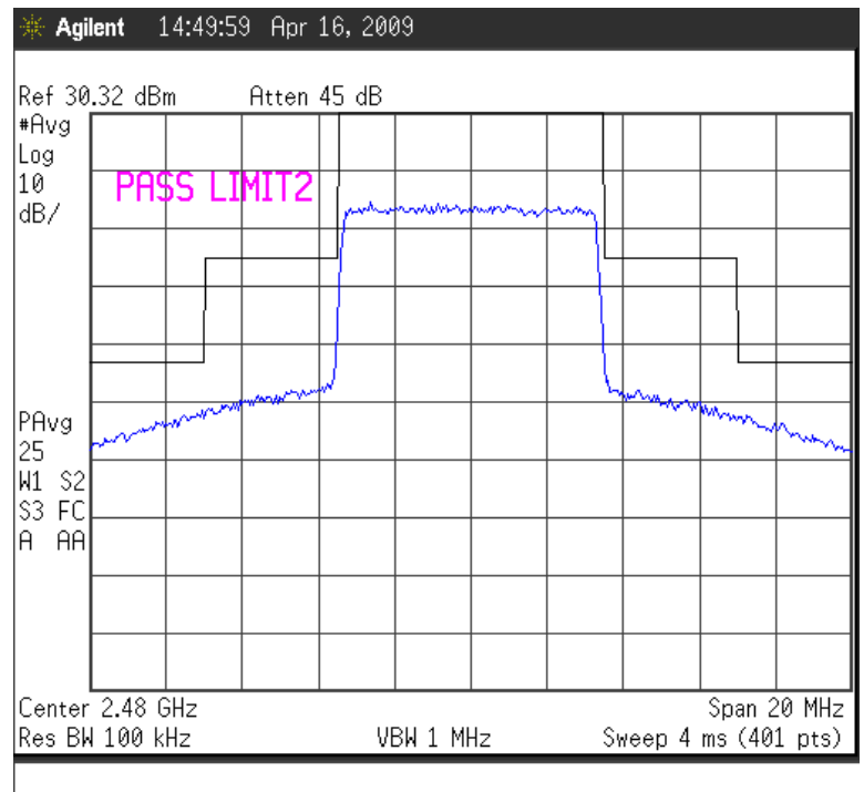
Fig. 15a Emission Mask Compliance TX Mode = DVB-T Emission: 7M0W7D Lower Band Edge
