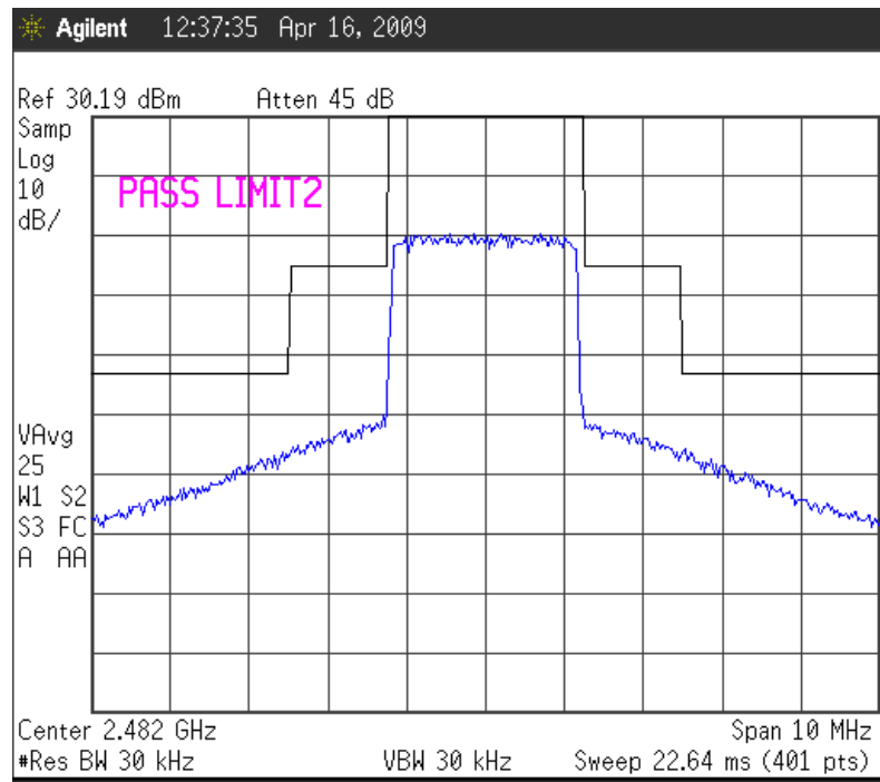
Fig. 13b Emission Mask Compliance TX Mode = DOMO-W Emission: 2M5W7D Upper Band Edge
