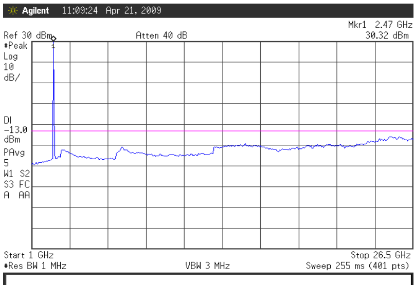
Fig. 9b Spurious Emissions Compliance 1GHz – 26GHz TX Mode = DVB-T Emission: 7M0W7D
