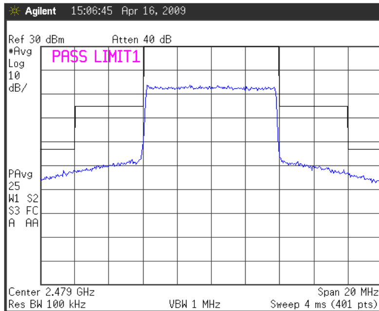
Fig. 16b Emission Mask Compliance TX Mode = DVB-T Emission: 8M0W7D Upper Band Edge
