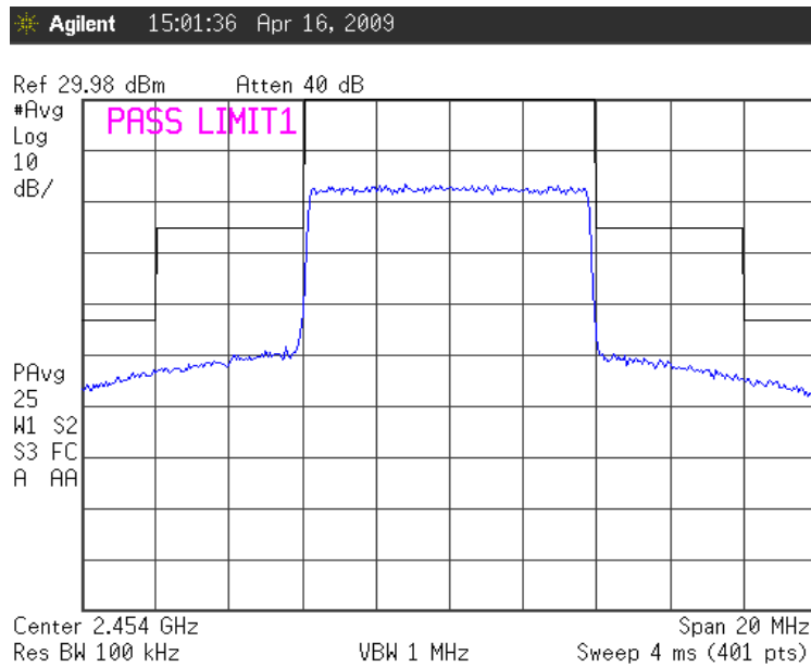
Fig. 16a Emission Mask Compliance TX Mode = DVB-T Emission: 8M0W7D Lower Band Edge
