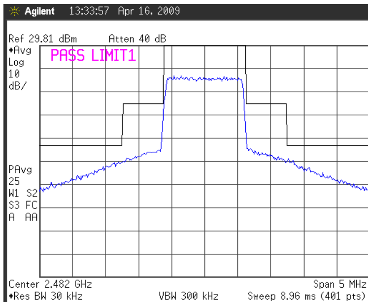
Fig. 12b Emission Mask Compliance TX Mode = DOMO-N Emission: 1M3W7D Upper Band Edge
