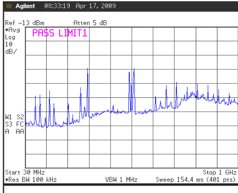
Fig. 7a Spurious Emissions Compliance 30MHz – 1GHz TX Mode = DOMO-W Emission: 2M5W7D
