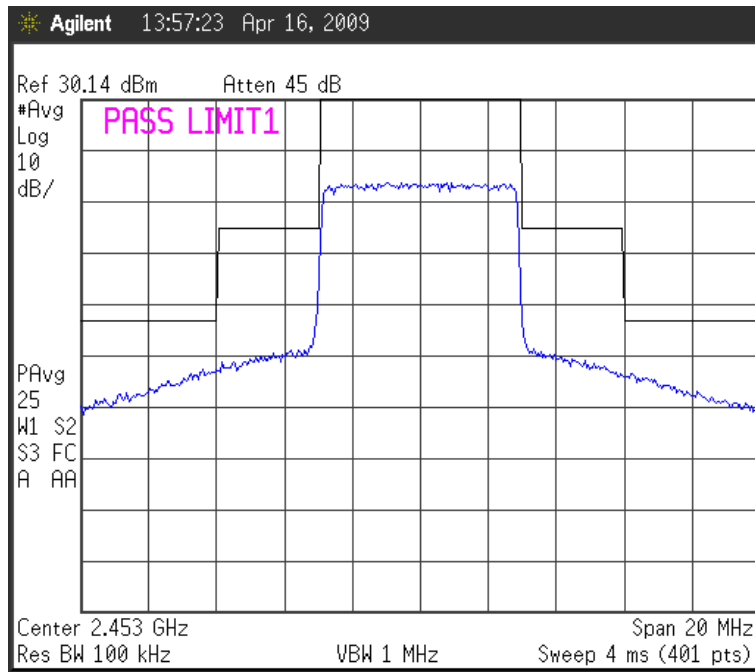
Fig. 14a Emission Mask Compliance TX Mode = DVB-T Emission: 6M0W7D Lower Band Edge
