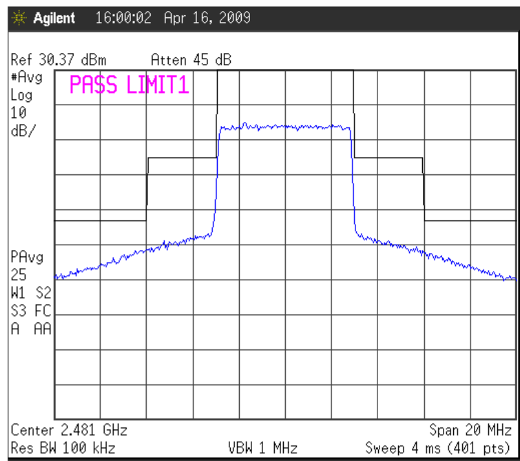
Fig. 14b Emission Mask Compliance TX Mode = DVB-T Emission: 6M0W7D Upper Band Edge
