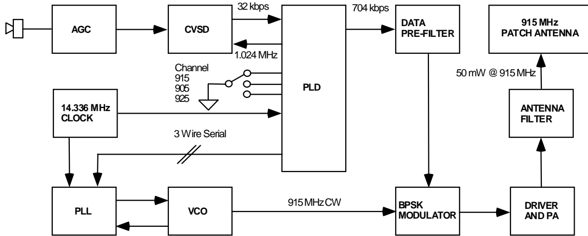
DSS900TX BLOCK DIAGRAM
