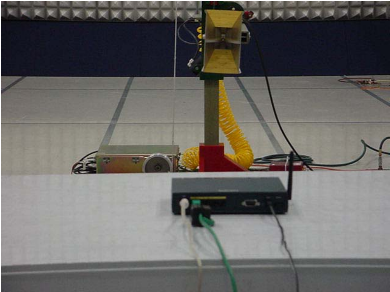
Radiated Emissions Test Setup Photo
