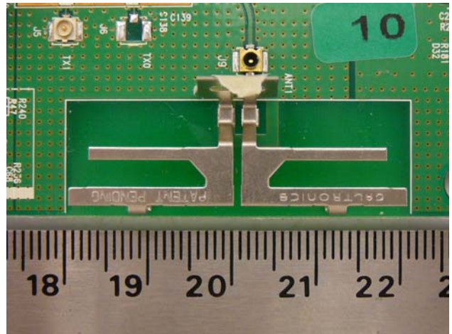
Antenna #1
