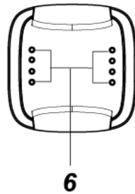
6. Charging & Programming Contact Plates 7. Type C Jack
