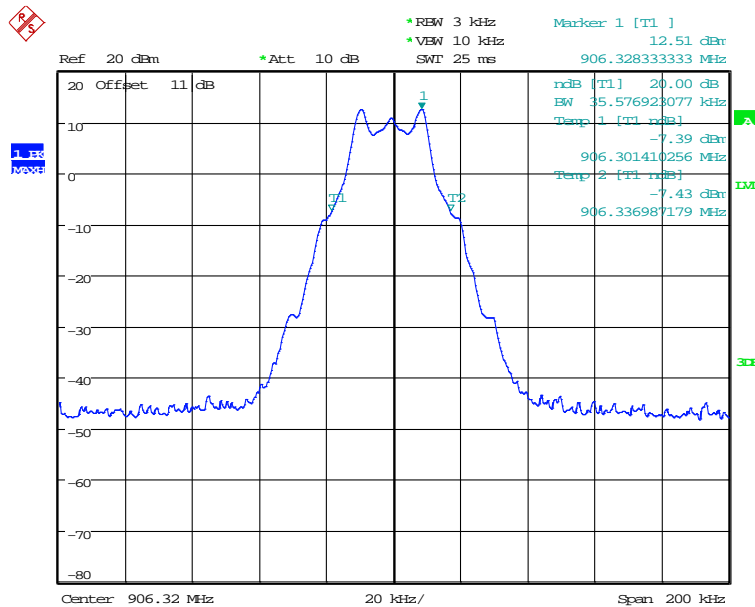
20DB BANDWIDTH 906.32MHz Date: 12.JUL.2024 11:49:54
